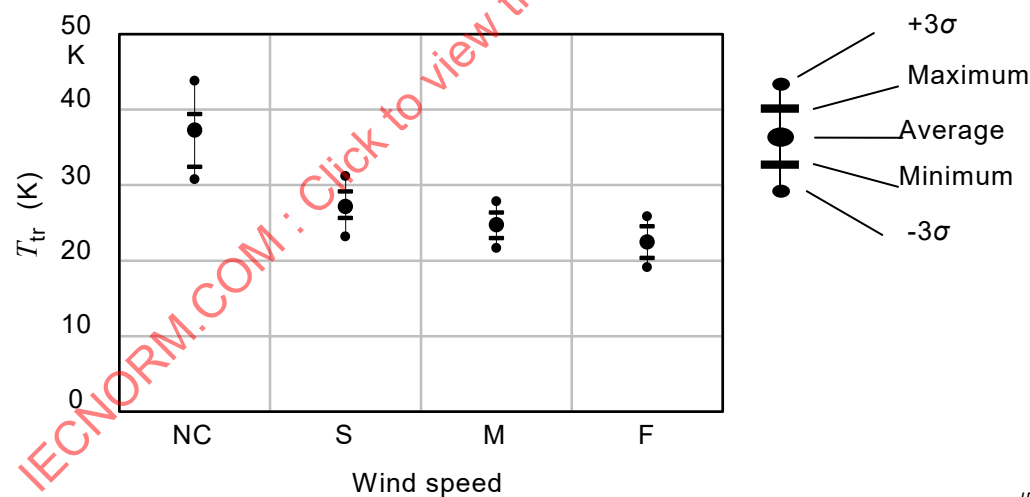
Figure D.8 – Wind speed and the terminal part temperature rise of the RR1608M
