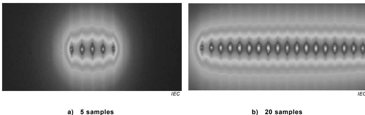
Figure C.3 – Infrared thermograph image in the same scale when power is applied to 5 samples and 20 samples
