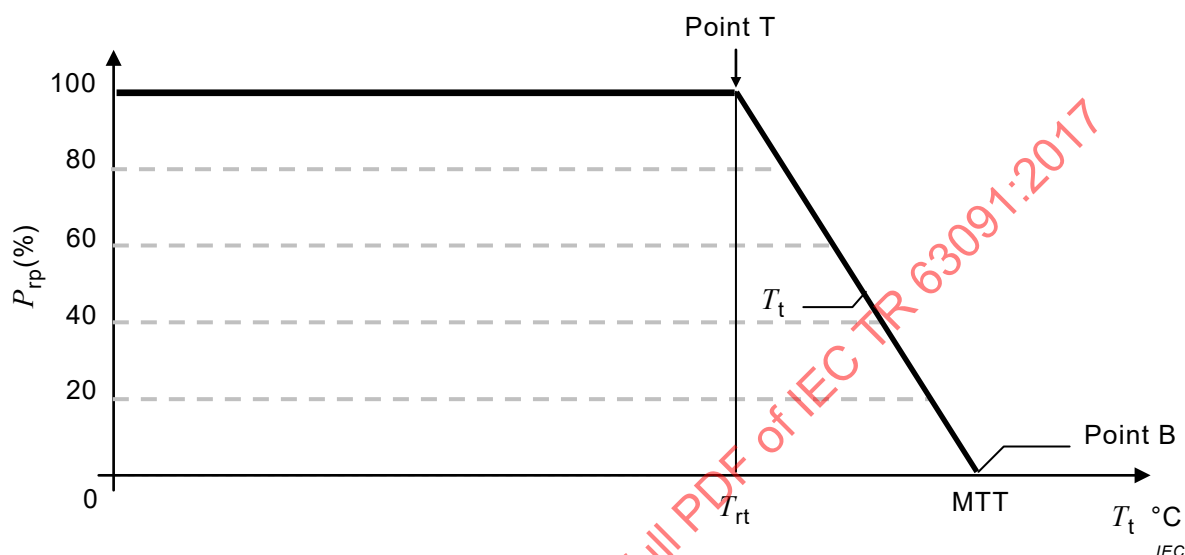
Figure E.3 – Derating curve based on the terminal part temperature
