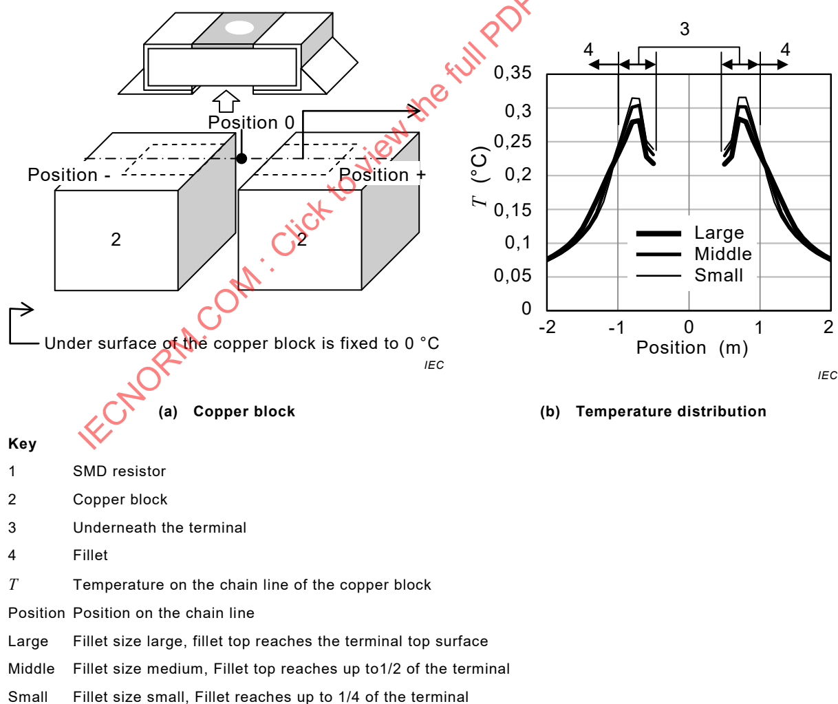
Figure H.3 – Temperature distribution of the copper block surface (calculated)
