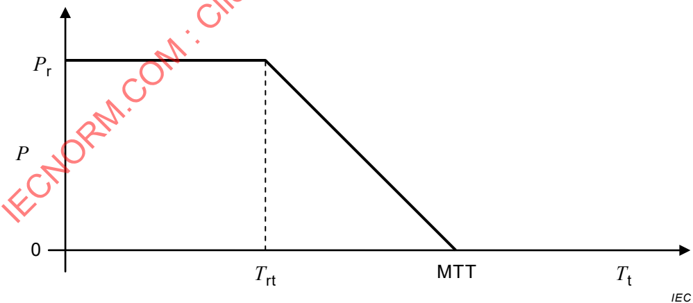
Figure 1 – Existing derating curve based on ambient temperature
