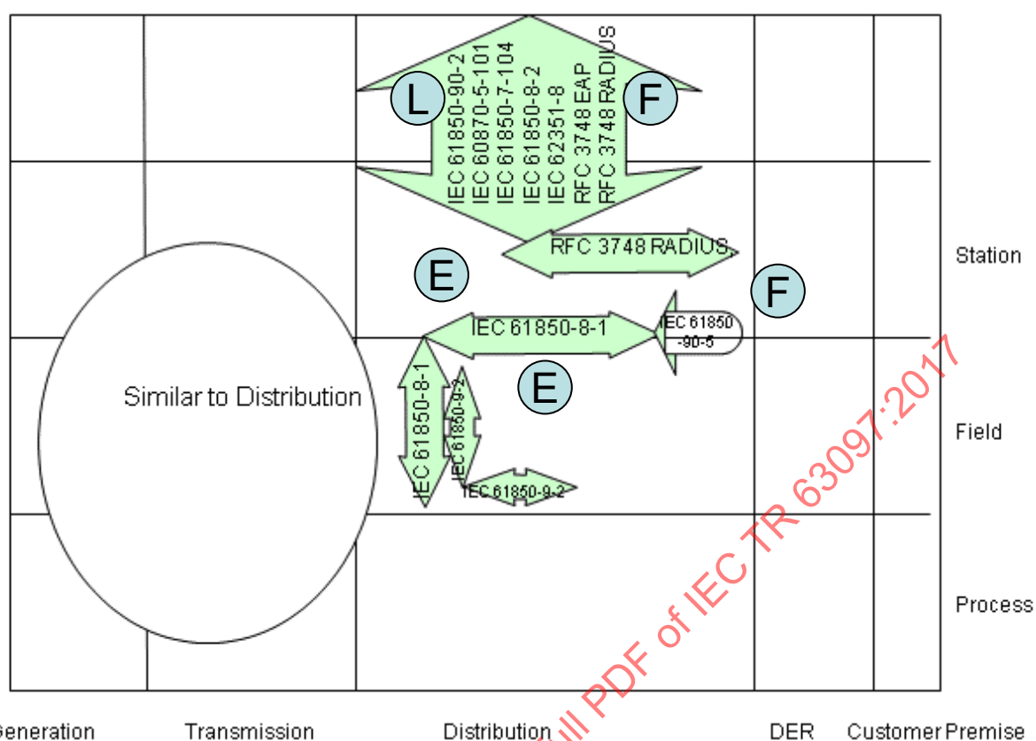
Figure 76 – Mapping of standards used in the AAA example on SGAM – Communication layer
