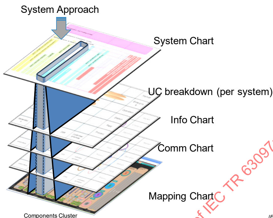
Figure 6 – Mapping principles of systems over the SGAM planes
