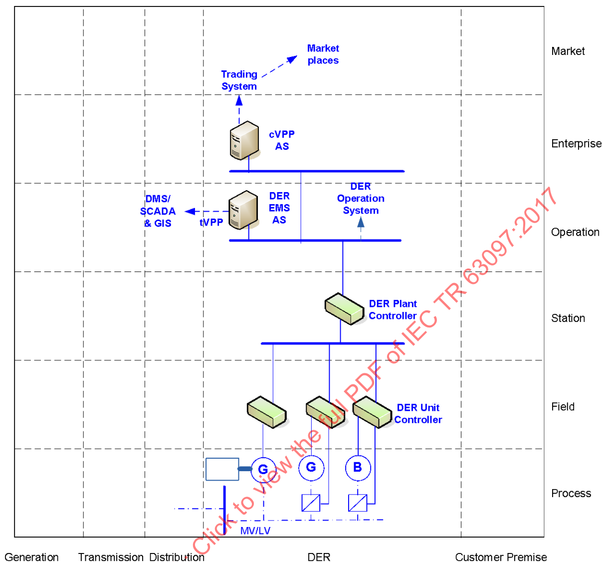
Figure 31 – DER management system – Component layer
