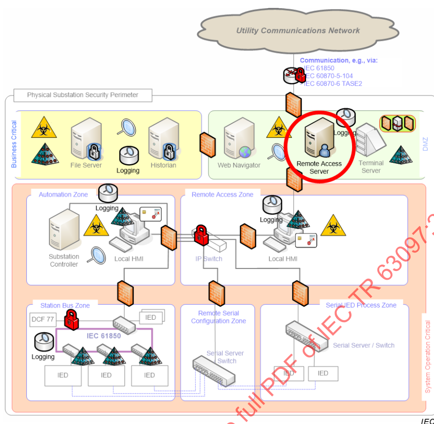
Figure 73 – AAA Example in a substation automation use case
