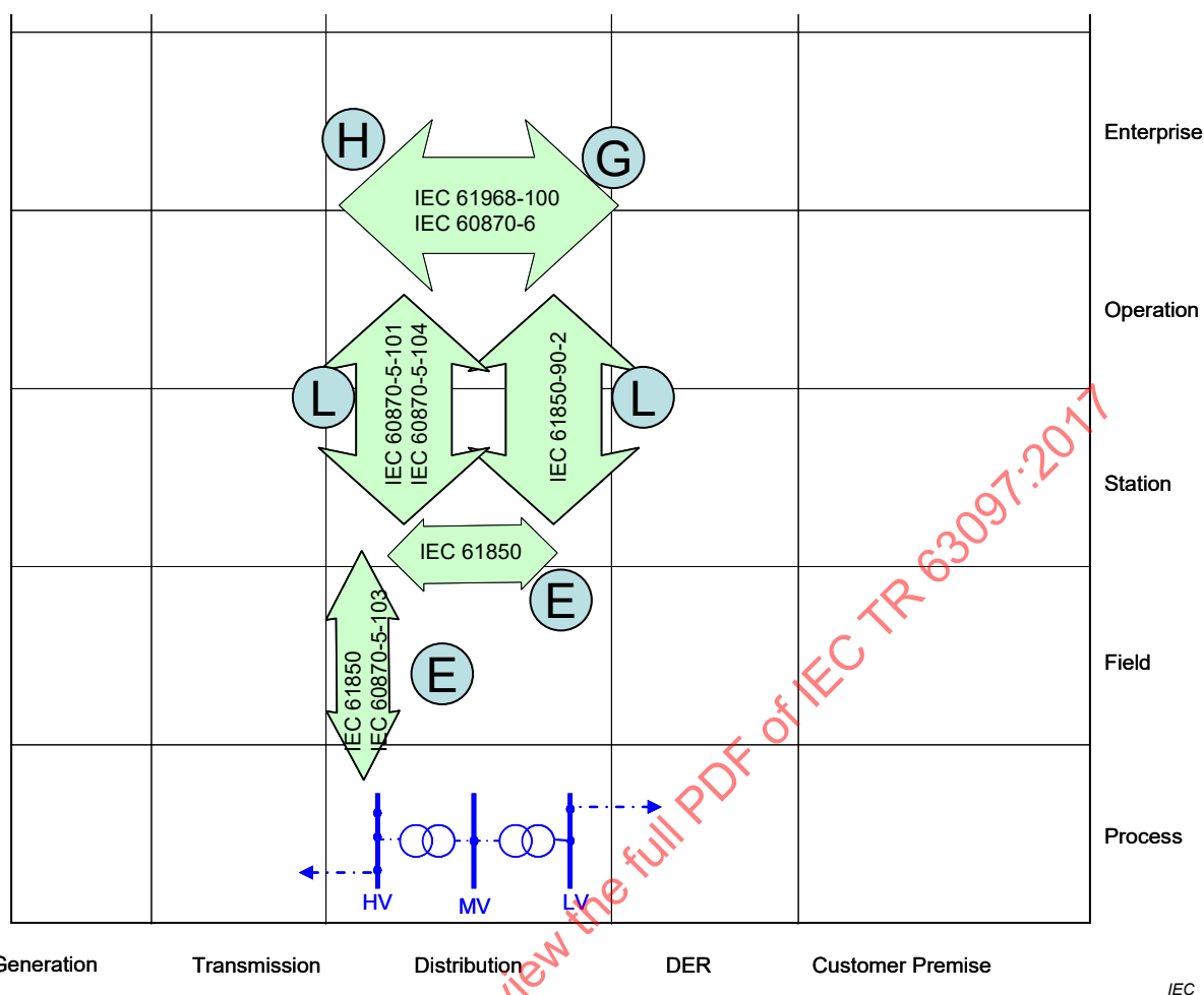
Figure 20 – DMS SCADA and GIS system – Communication layer
