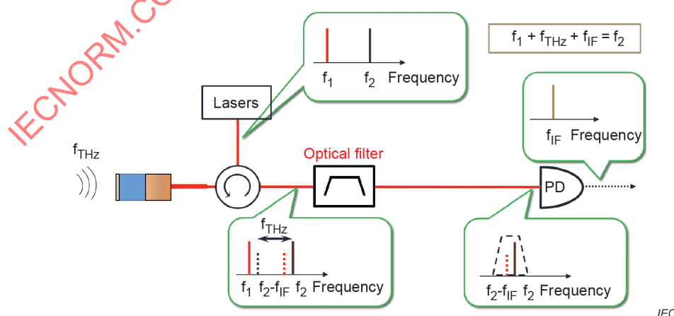
Figure 3 – Principle of the non-polarimetric EO frequency down-conversion technique
