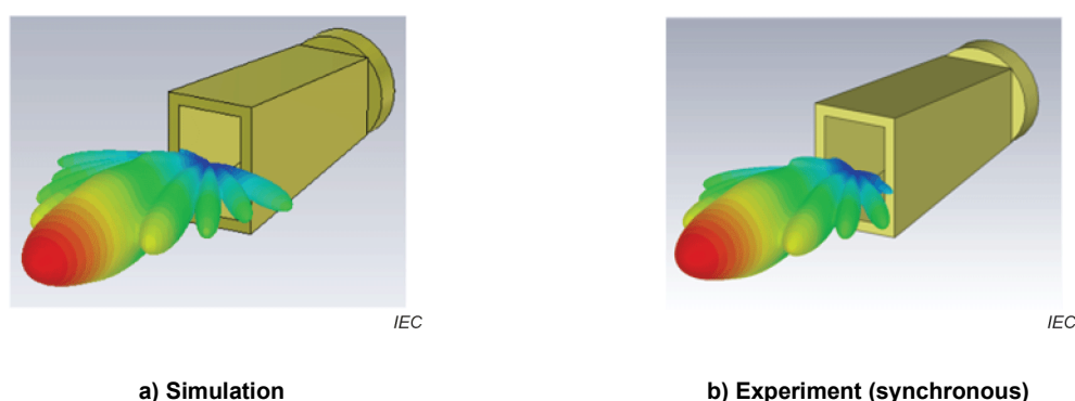
Figure 7 – Far-field pattern calculated from the near-field measured by the synchronous system
