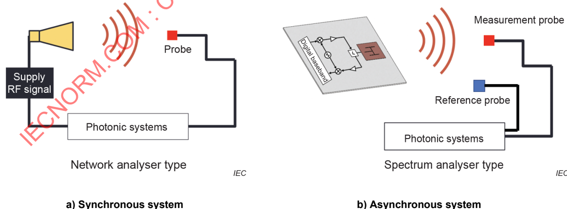
Figure 1 – Proposed measurement system
