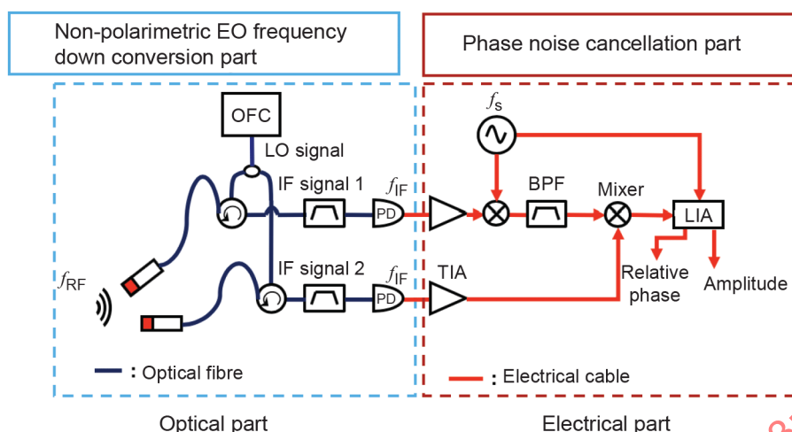
Figure 9 – Schematic diagram of the asynchronous system based on the phase noise cancelling technique
