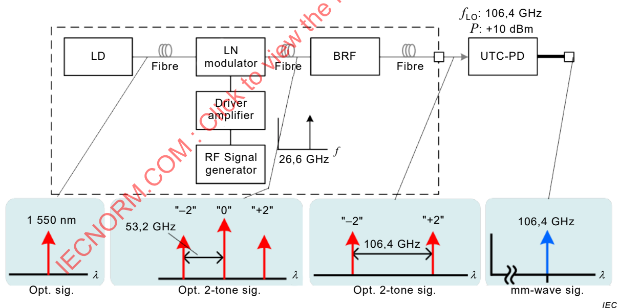
Figure 6 – RoF Sig Gen block diagram
