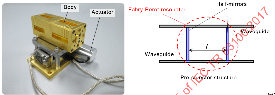
Figure 3 – Fabry-Perot tunable filter
