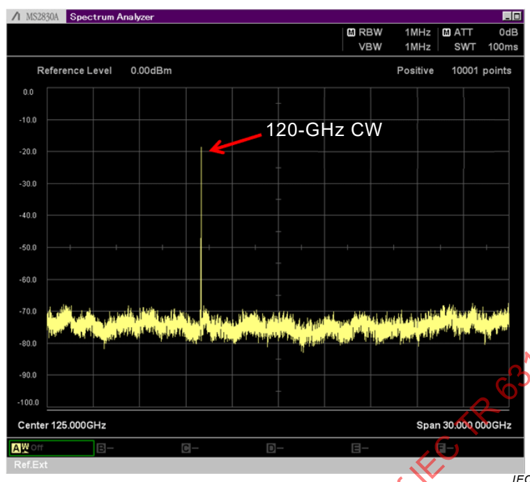
Figure 11 – Spectrum measurement
