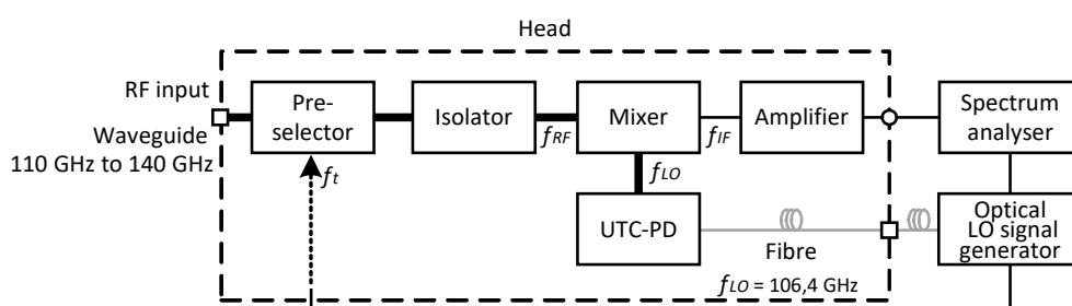
Figure 2 – 100-GHz spectrum analyser block diagram
