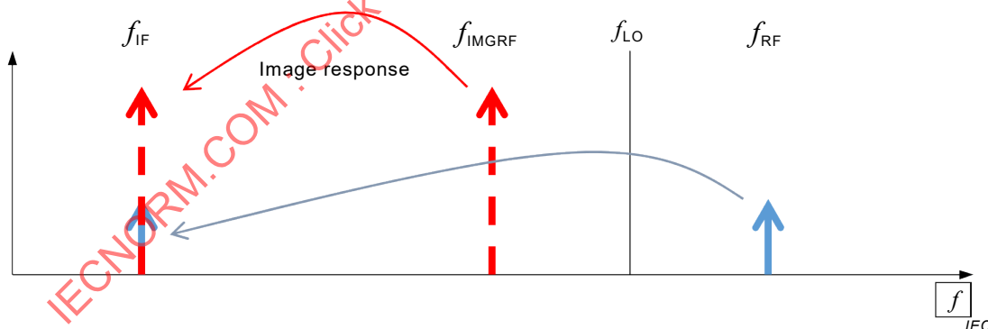
Figure 12 – Image response
