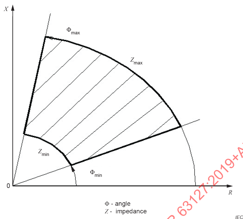
Figure 3 – Sector diagram of system harmonic impedance
