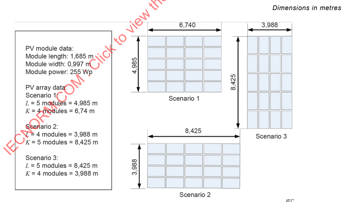
Figure 26 – Array configuration for horizontal double tracking
