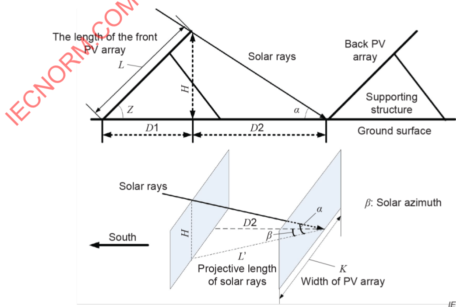
Figure 8 – Relationship of solar beam and PV array
