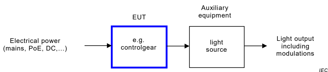
Figure 5 – Controlgear testing
