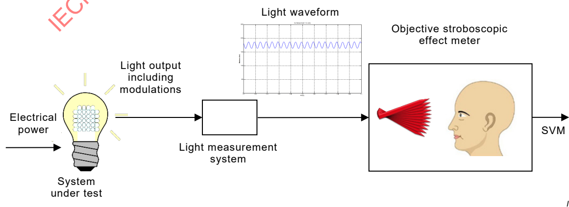
Figure 1 – Schematic of the stroboscopic effect measurement method
