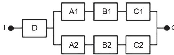
Figure 3 – General series-parallel (redundancy) reliability block diagram
