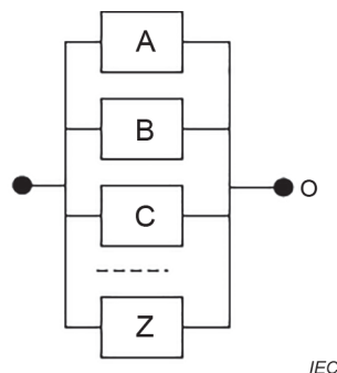
Figure 2 – Parallel reliability block diagram
