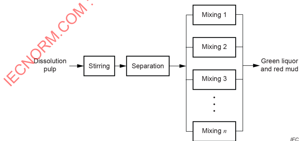
Figure A.3 – Settling and washing process for aluminum smelting automation system
