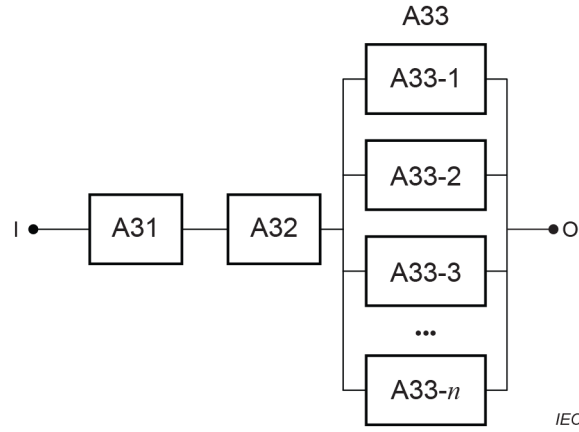
Figure A.4 – Block diagram for settling and washing process
