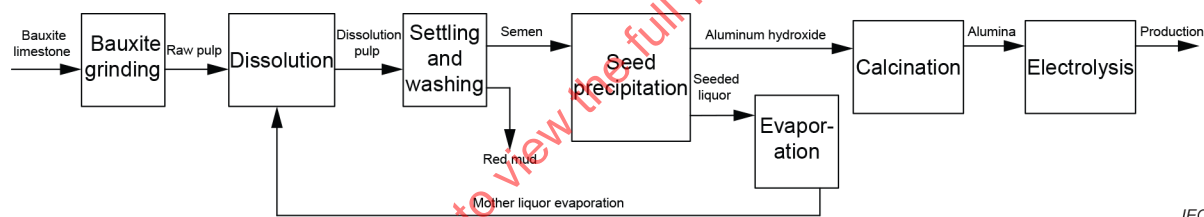
Figure A.1 – A typical process automation system (aluminum smelting)
