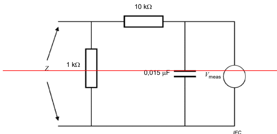
Figure 4 — Simulated body impedance for contact current measurements shown in IEEE C95.3 [27]
