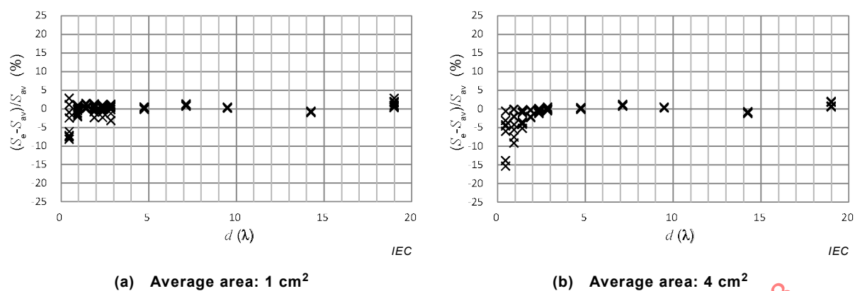
Figure D.4 – Difference of S_e to S_{av} for all antennas (%)
