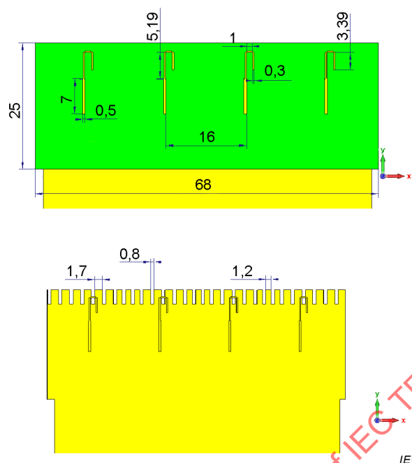
Figure H.2 – Antenna geometry
