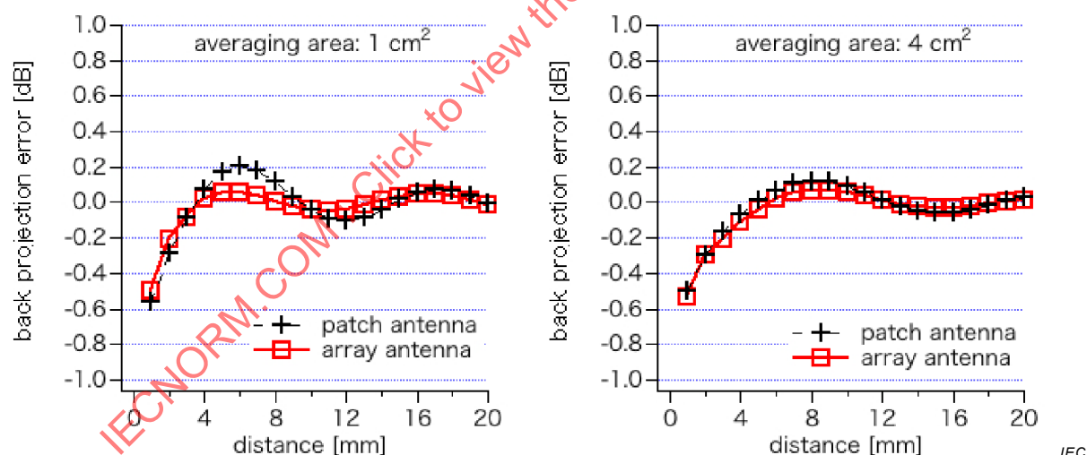
Figure F.1 – Comparison of maximum values of S_{av} between the computational simulation and back projection at 30 GHz
