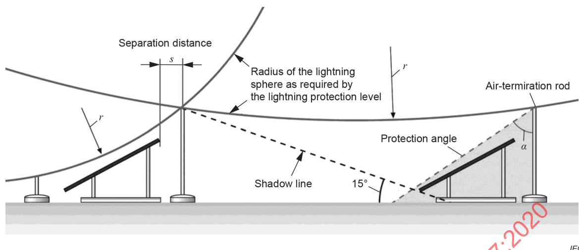
Figure 6 – Example for the design of the air-termination system for a PV power supply system
