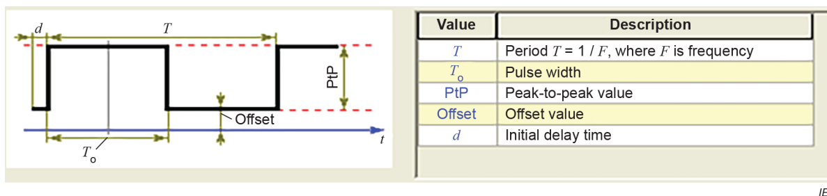
Figure 3 – Signal “Sig2”: Rectangular wave
