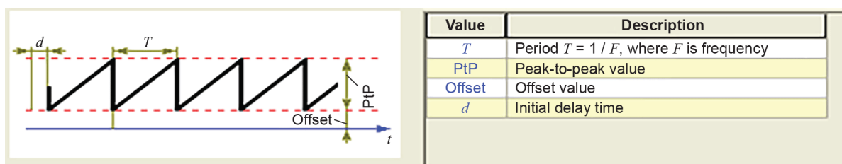
Figure 6 – Signal “Sig5”: Upper half sine wave
