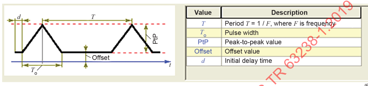
Figure 4 – Signal “Sig3”: Symmetrical triangular wave
