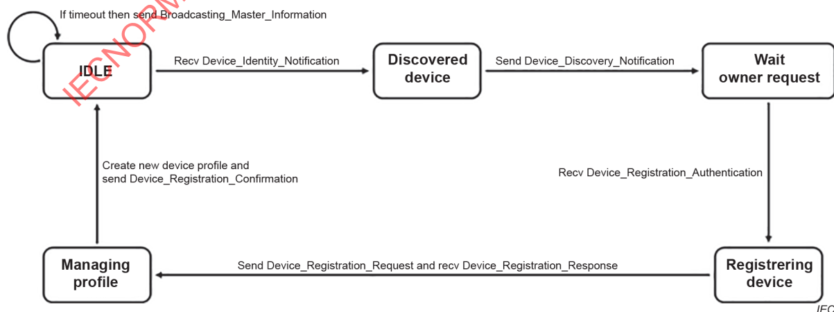
Figure 8 – State transitions of CCIS master in device registration
