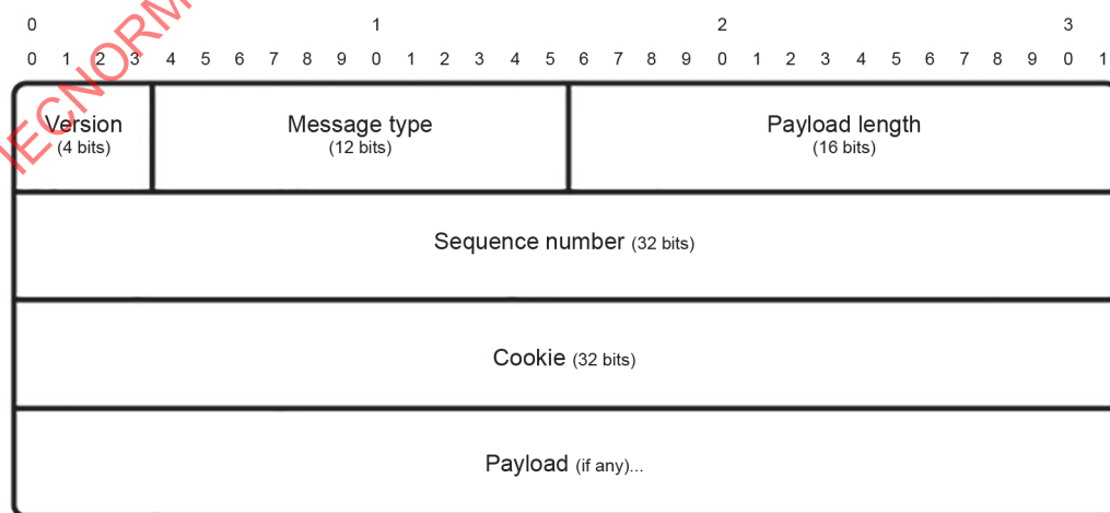
Figure 2 – Message format of CCIS protocol
