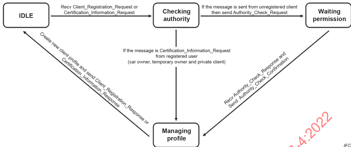
Figure 7 – States transitions of CCIS master in client registration and certification
