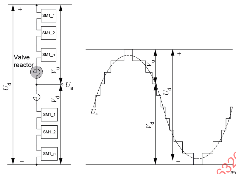
Figure 10 – Single-phase voltage waveform on the AC side
