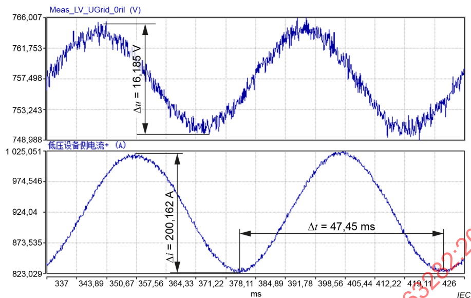
Figure B.2 – The voltage and current oscillation waveform on \pm 375 V bus
