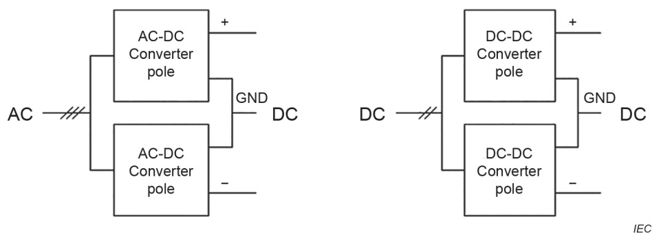
Figure 10 – A schematic of a bipolar system (the CIGRE B4 DC test system)
