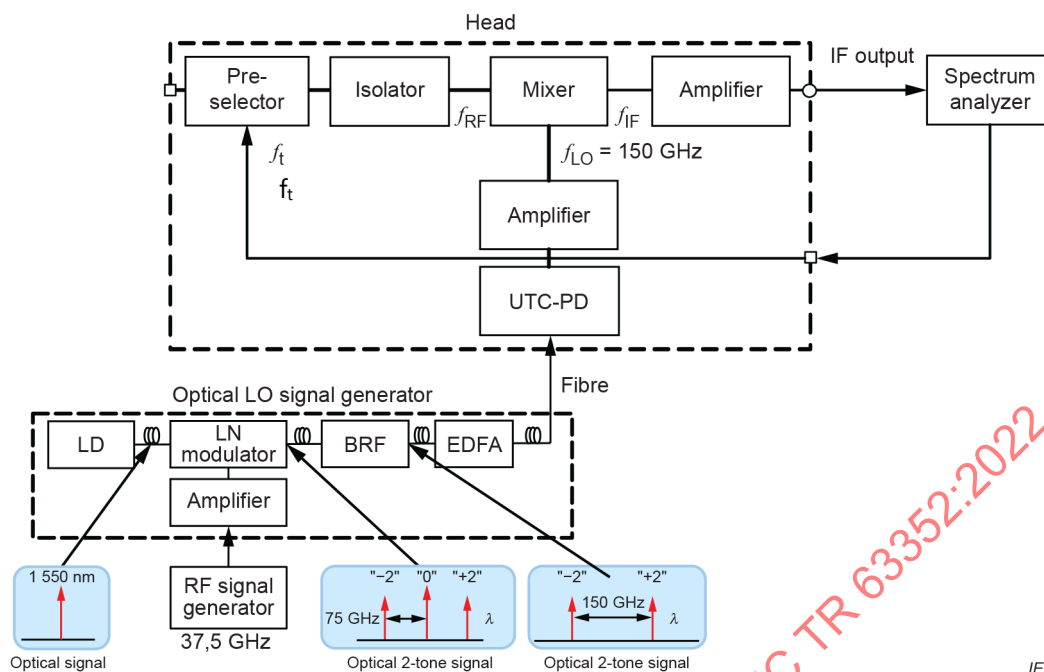
Figure 5 – 300-GHz spectrum analysis system with optical local signal generation
