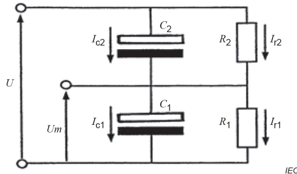
Figure 4 – Voltage sharing analysis
