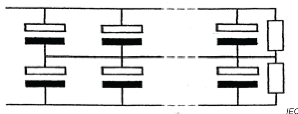
Figure 2 – Common centre connection
