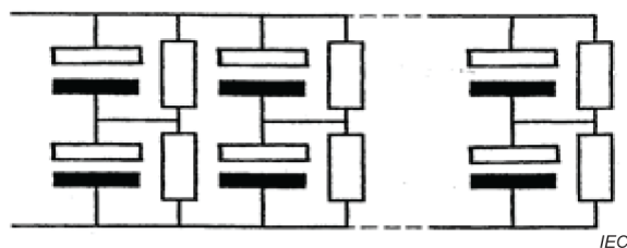
Figure 1 – Individual balancing resistors
