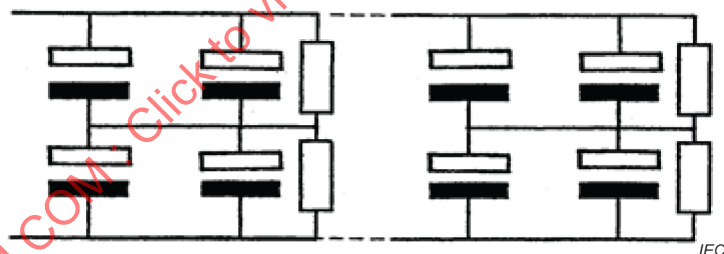
Figure 3 – Group-balancing resistors
