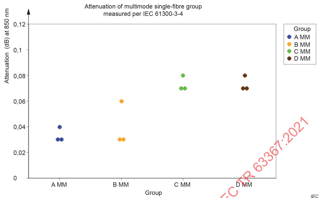
Figure B.1 – Initial attenuation of multimode single-fibre specimens
