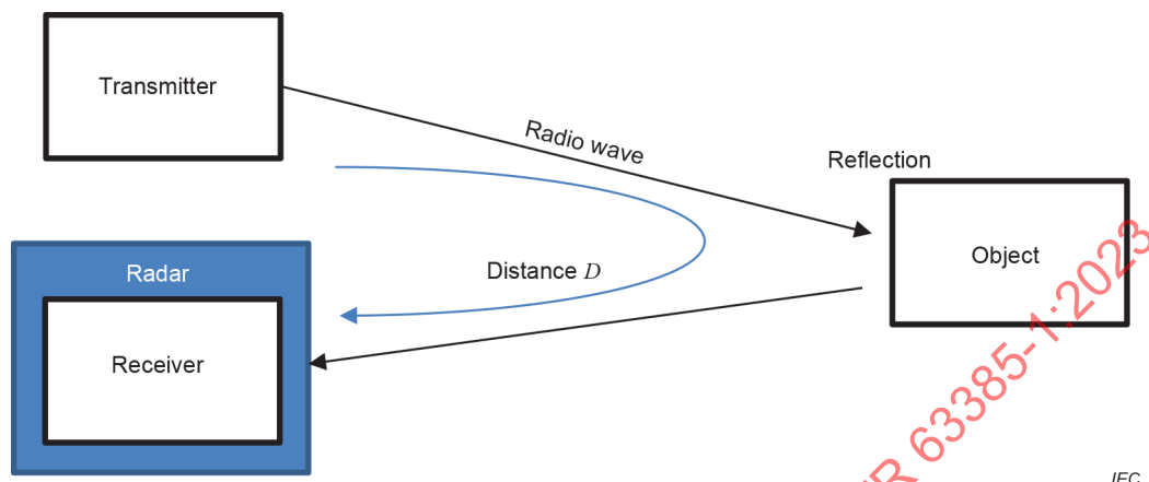
Figure 6 – Principle of passive radar system
