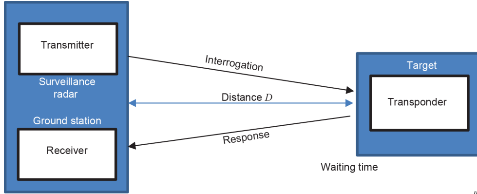
Figure 5 – Principle of secondary surveillance radar system
