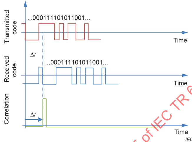
Figure 4 – Time measurement using correlation calculation by digital codes
