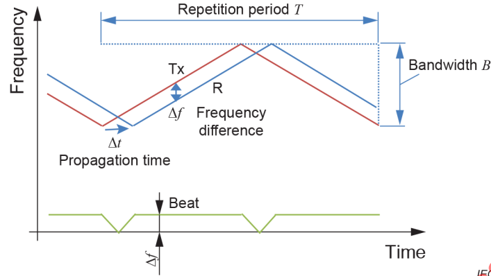
Figure 3 – Frequency sweep pattern and beat frequency of transmission and reception for linear FMCW radar
