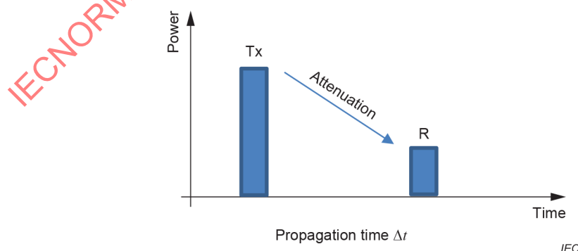
Figure 2 – Waveform and timing of transmission and reception for a pulsed radar system
