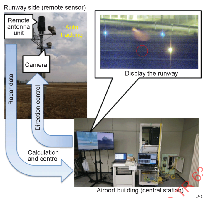
Figure 8 – Foreign object and debris detection system
