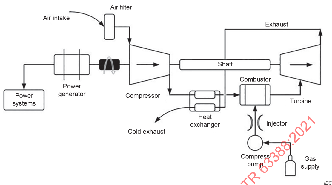
Figure 14 – CHP system based on micro gas turbine
