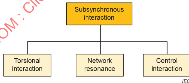
Figure 5 – Reclassification of subsynchronous interactions based on the interaction mechanism
