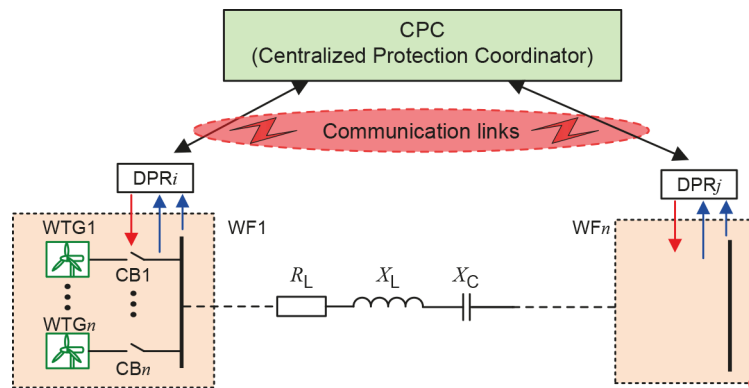
Figure 39 – A system-wide SSCI mitigation scheme based on selective tripping of WTGs
