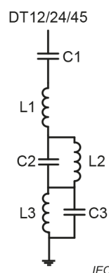
Figure 36 – Three tuned DC filters TT12/24/45
