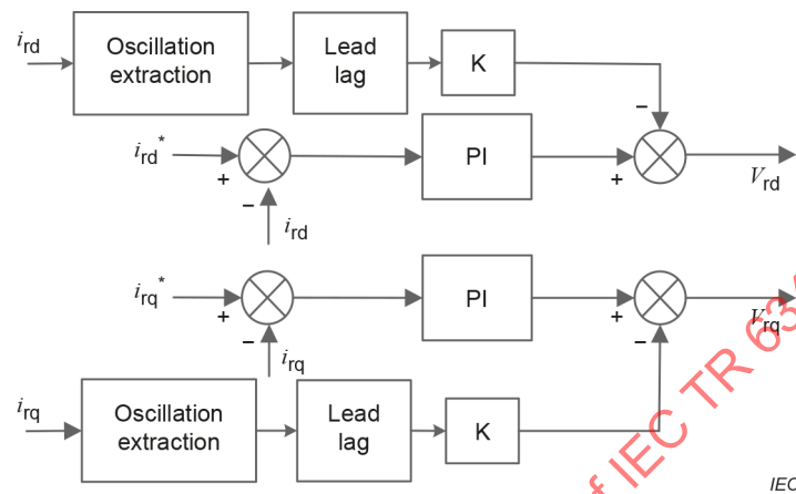
Figure 44 – Control diagram of the virtual resistor for DFIG's RSC controllers
