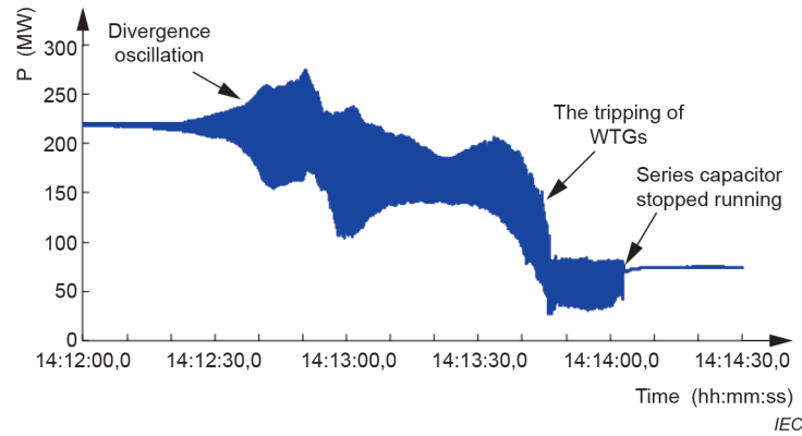
Figure 14 – Power flow measured at the 200 kV side of the Guyuan step-up transformer
