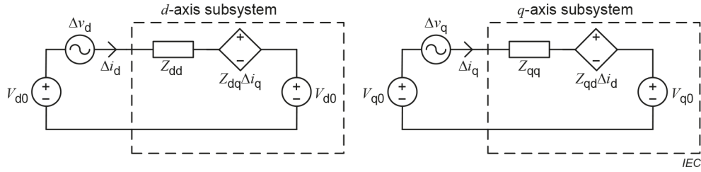
Figure 24 – Three-phase subsystem represented in the dq domain using equivalent small-signal impedance
