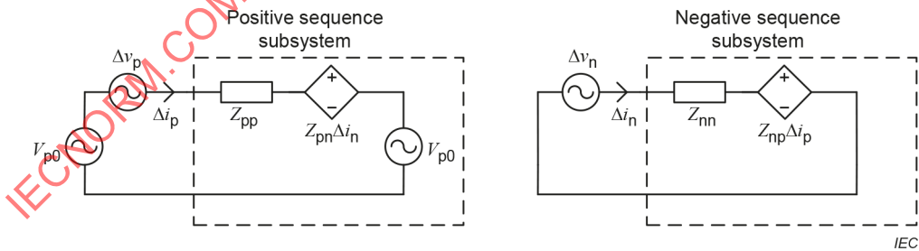
Figure 25 – Three-phase subsystem represented in the sequence domain using equivalent small-signal impedance
