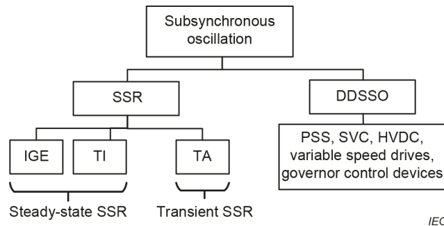
Figure 3 – Terms and classification of SSR by IEEE [13]
