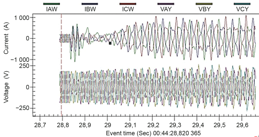
Figure 8 – Oscilloscope record of the 2009 SSCI event in the ERCOT system [19]
