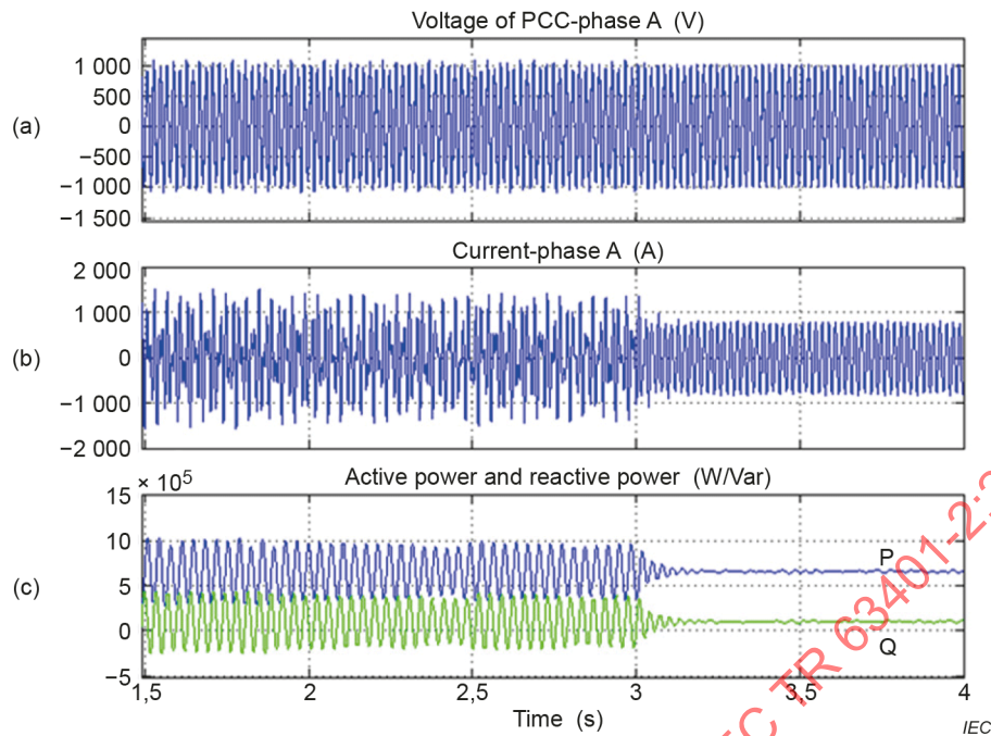
Figure 42 – SSCI mitigation by increasing the K_p of the inner controllers of the GSC (a) voltage at PCC (b) current phase-A (c) active and reactive power
