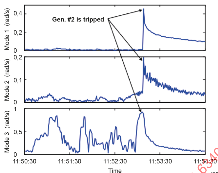
Figure 22 – Torsional speed of modes 1 to 3 of unit #2 in Plant M
