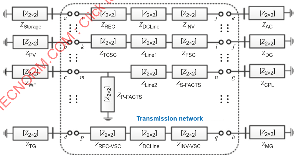
Figure 29 – The unified dq -frame INM of a typical power system
