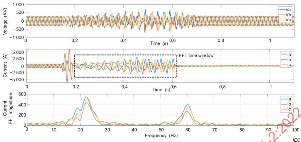
Figure 11 – Event#2 September 27, 2017: current, voltage and frequency spectrum of the current during the SSCI event [24]
