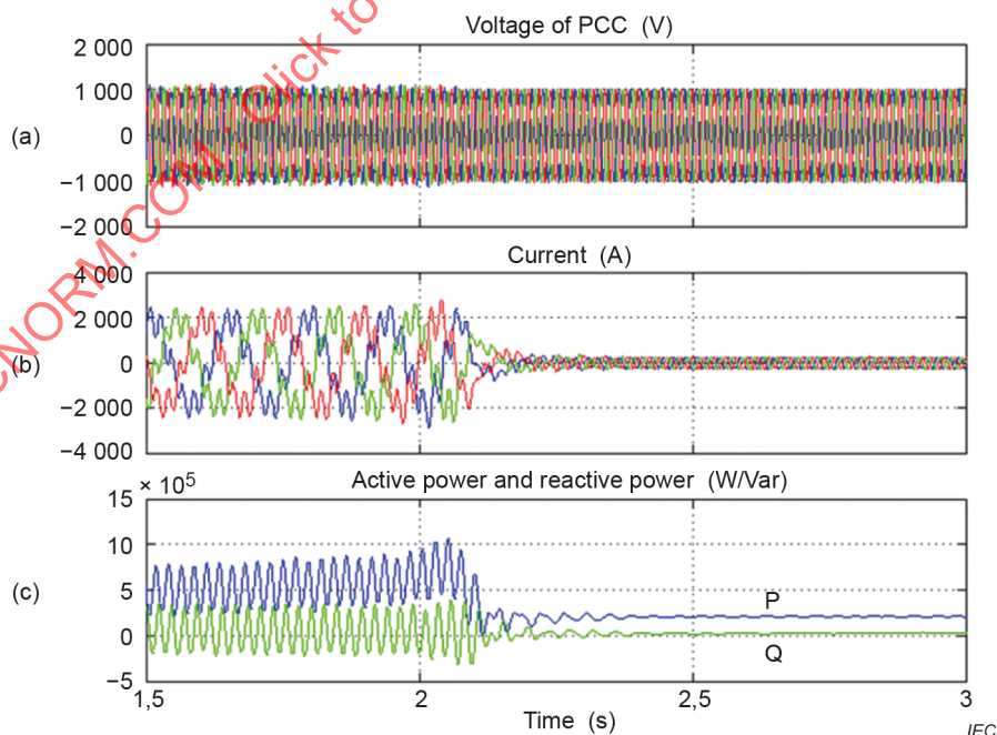
Figure 45 – The SSCL damped out when the virtual resistor is enabled at 2 seconds in simulation (a) voltage at PCC (b) current phase-A (c) active and reactive power
