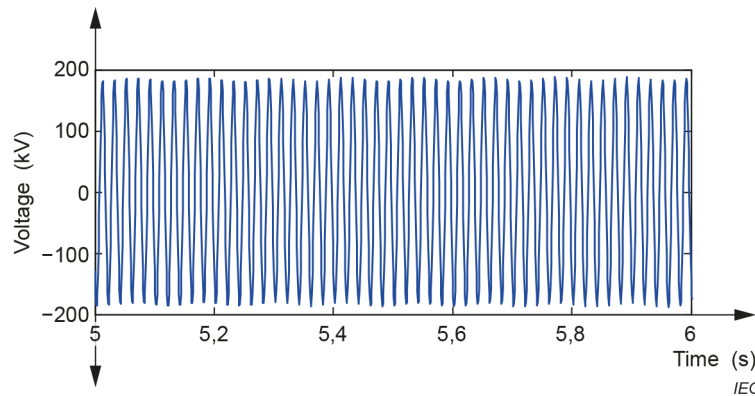
(a) Phase A voltage
