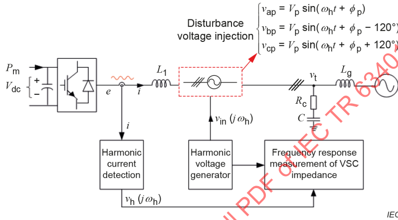
Figure 26 – Impedance measurement in a simple system
