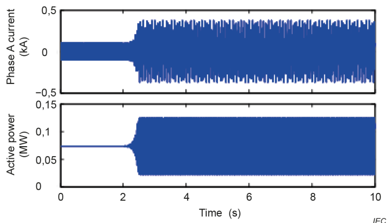
Figure 18 – Current (upper plot) and active power (lower plot)
