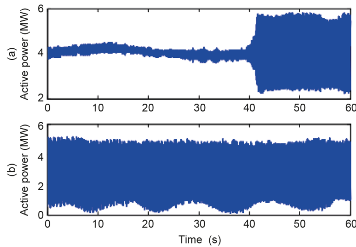
Figure 20 – Field measured active power of a wind farm (a) From 09:46 to 09:47 (b) From 11:52 to 11:53
