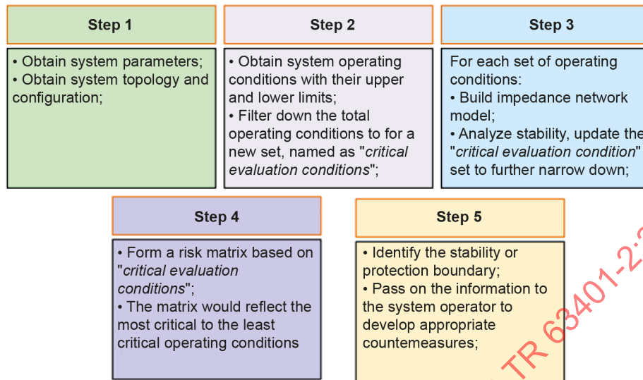
Figure 30 – Recommended guidelines for the SSCI stability analysis of a real-world wind power system
