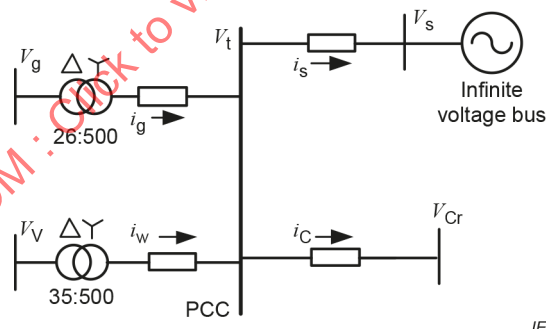
Figure 37 – The common electrical network
