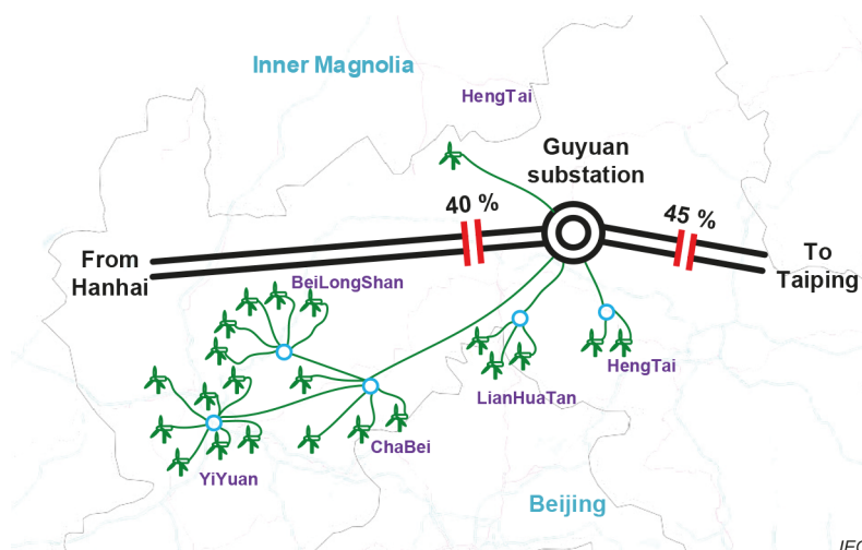
Figure 13 – Geographical layout of the Guyuan wind power system, Hebei Province, China
