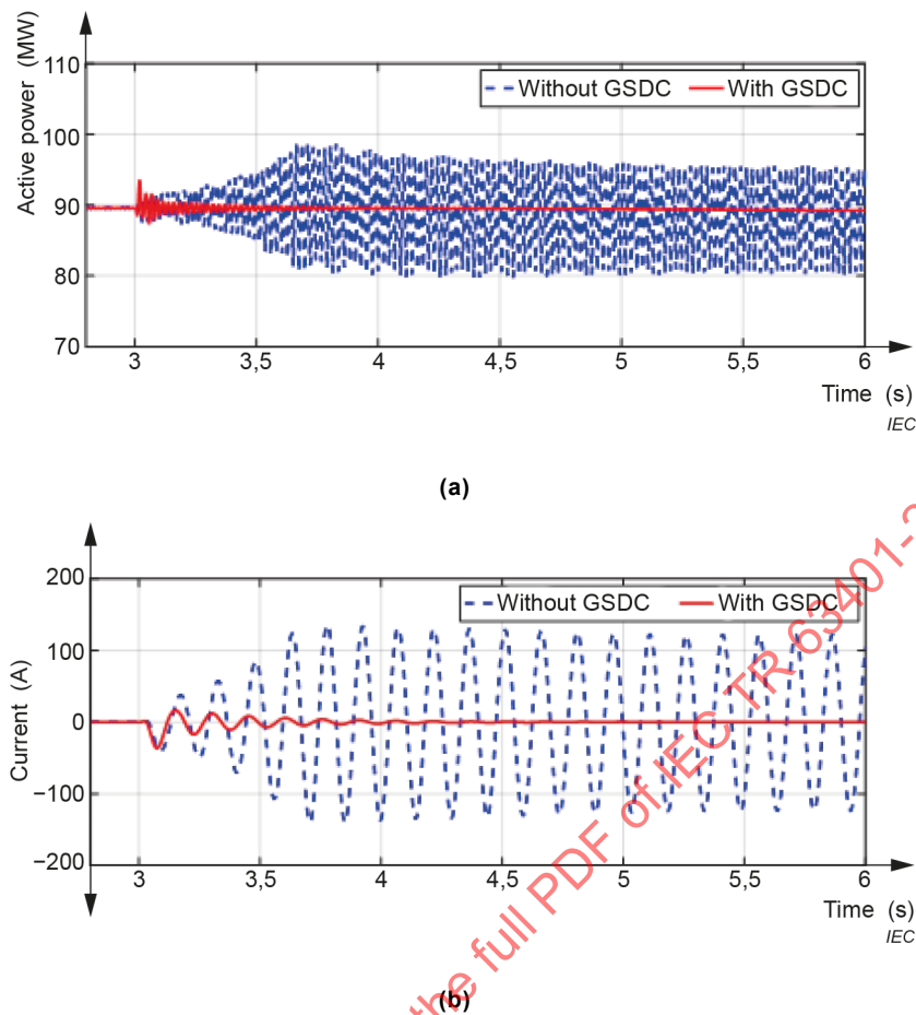
Figure 41 – CHIL test results of GSDC (a) active power (b) subsynchronous current
