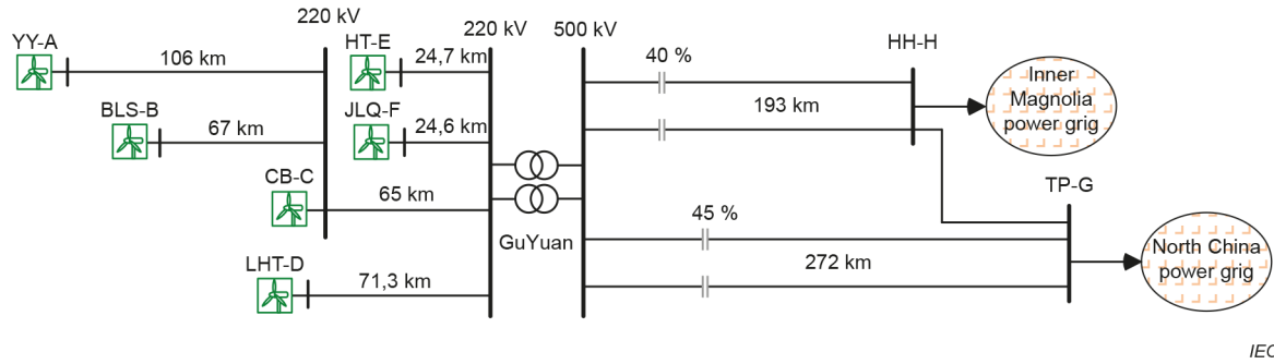
Figure 31 – One-line diagram of the proposed benchmark model adopted from the Guyuan wind power system
