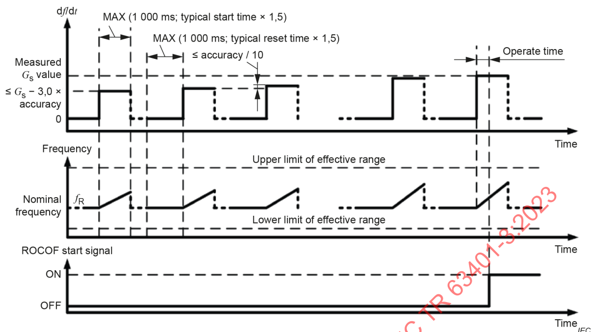
Figure 21 – Example of test method for positive ROCOF function
