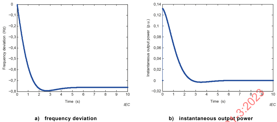
Figure 9 – Controlled contribution of electrical power provided by ROCOF-based FFR
