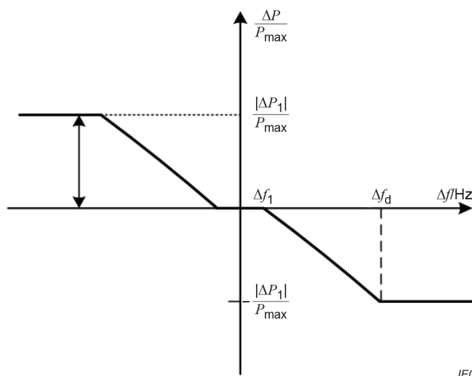
Figure 10 – The controlled contribution of electrical power provided by deviation-based FFR
