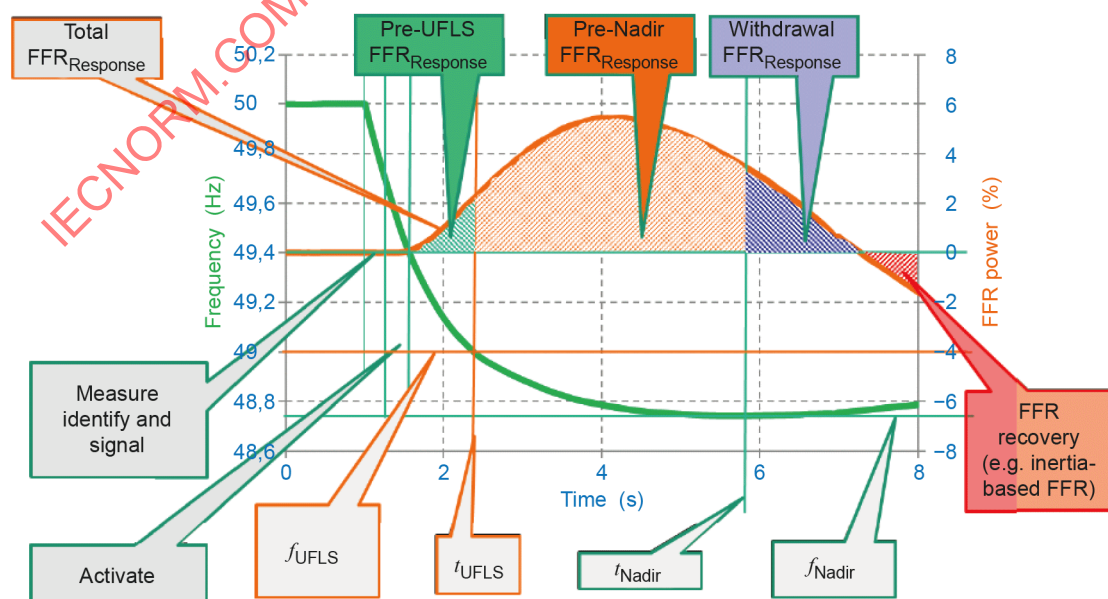
Figure 14 – Time elements of FFR
