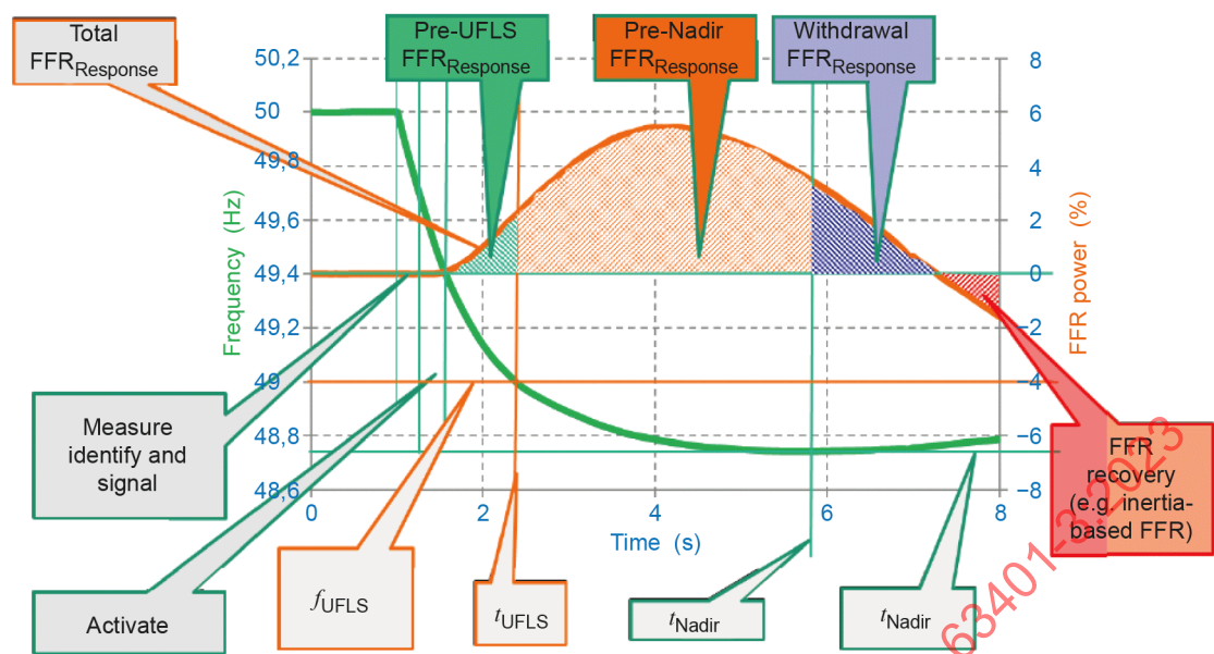
Figure 2 – Time elements of FFR
