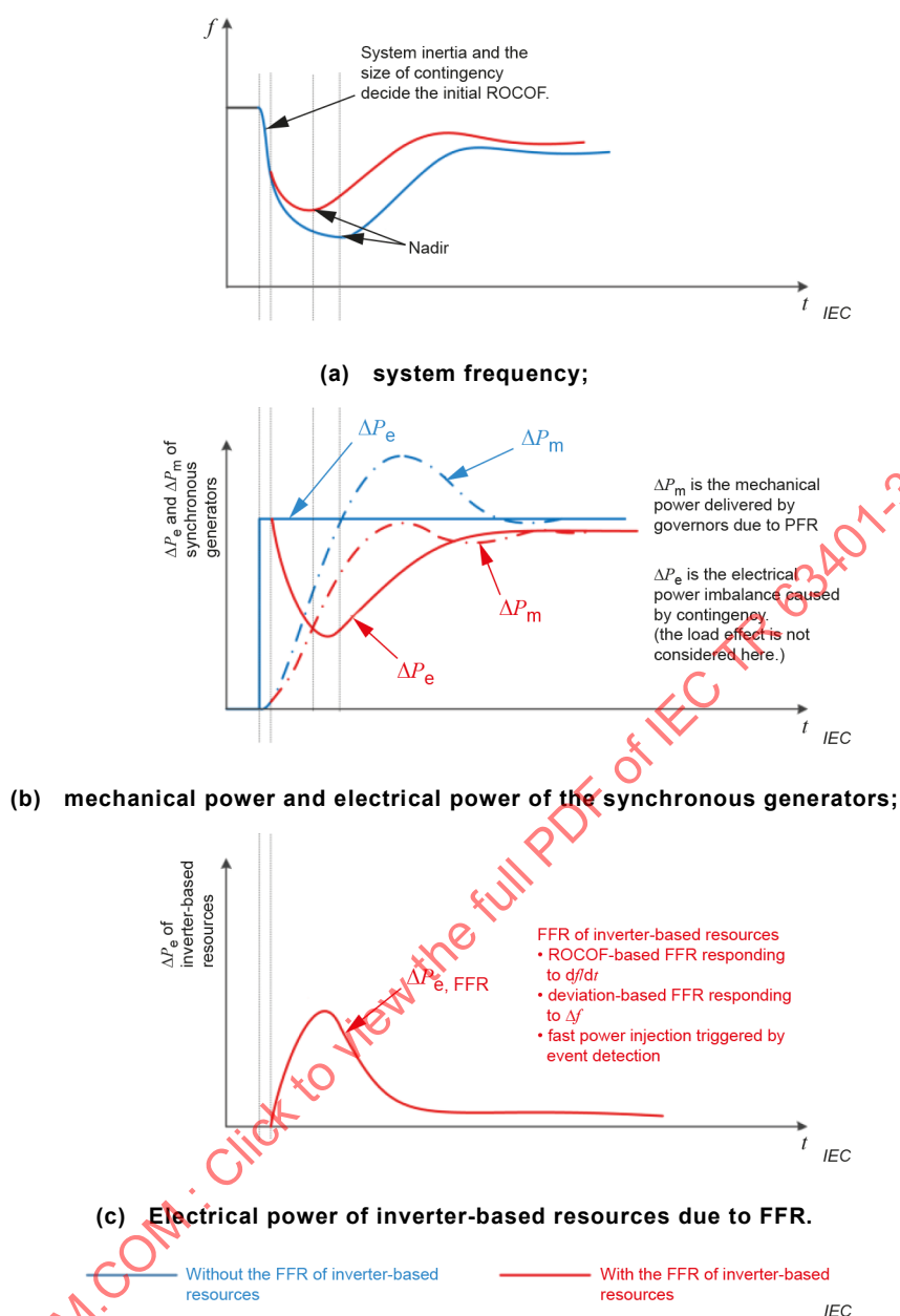
Figure 3 – Impact mechanism on system frequency by FFR
