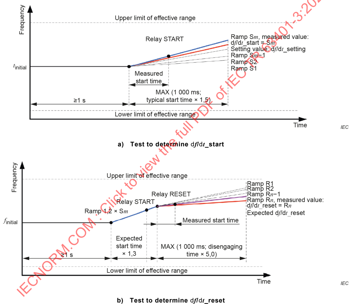
Figure 22 – Test method for measurement of reset value for ROCOF functions: example for positive ROCOF function
