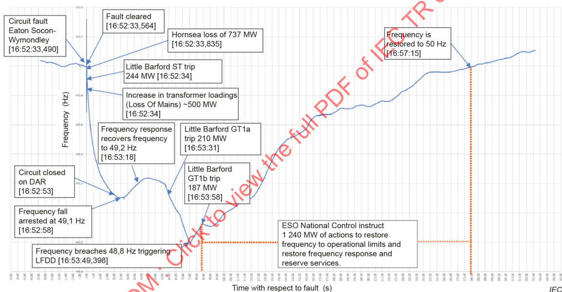
Figure 6 – Frequency response in blackout in Great Britain power grid on 9 August 2019
