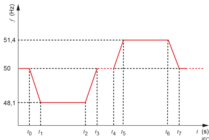
Figure 16 – Test slope curve for ROCOF-based FFR
