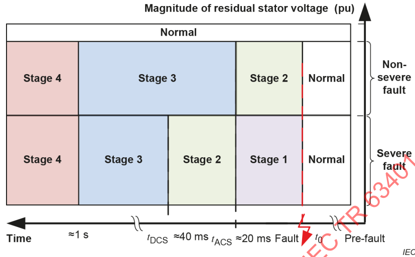
Figure 19 – FRT solutions of a DFIG-based WT during grid fault
