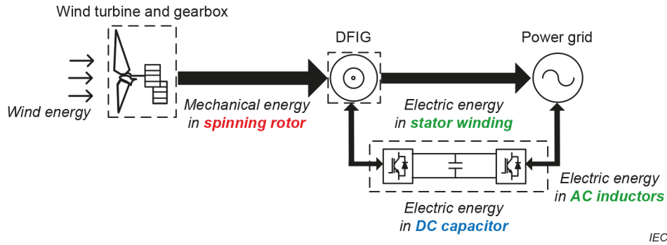
Figure 16 – Energy flow and ESEs of a DFIG-based WT in normal operation
