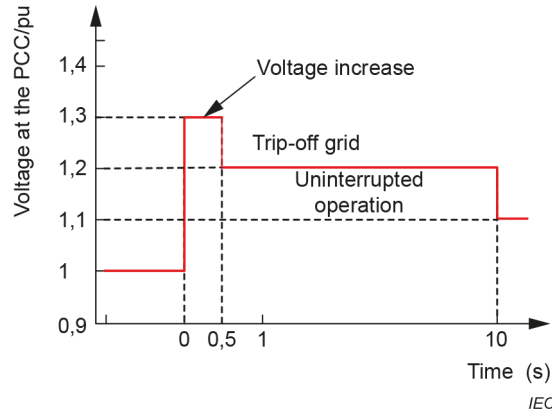
Figure 7 – Over voltage ride through requirements for photovoltaic power stations in China
