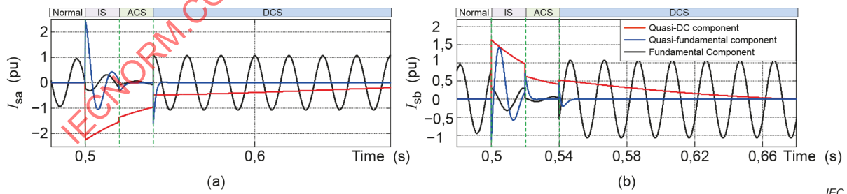
Figure 20 – The identified components of fault currents by the analytical expression
