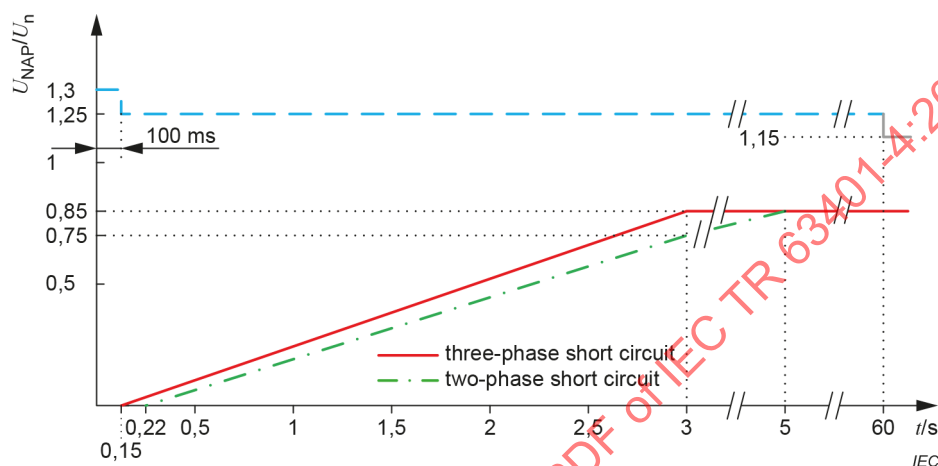
Figure 8 – Voltage ride through requirements for type II power stations according to VDE-AR-N-4120
