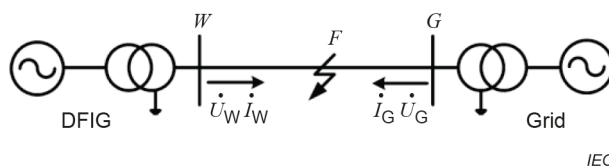
Figure 29 – Wind power integration system
