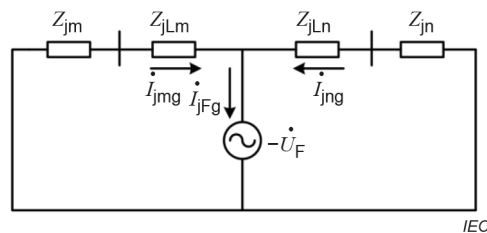
Figure 31 – Fault component network
