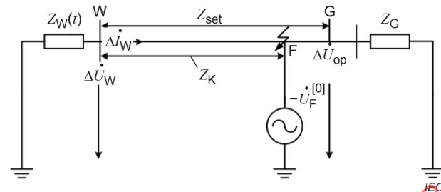
(b) Fault component network
