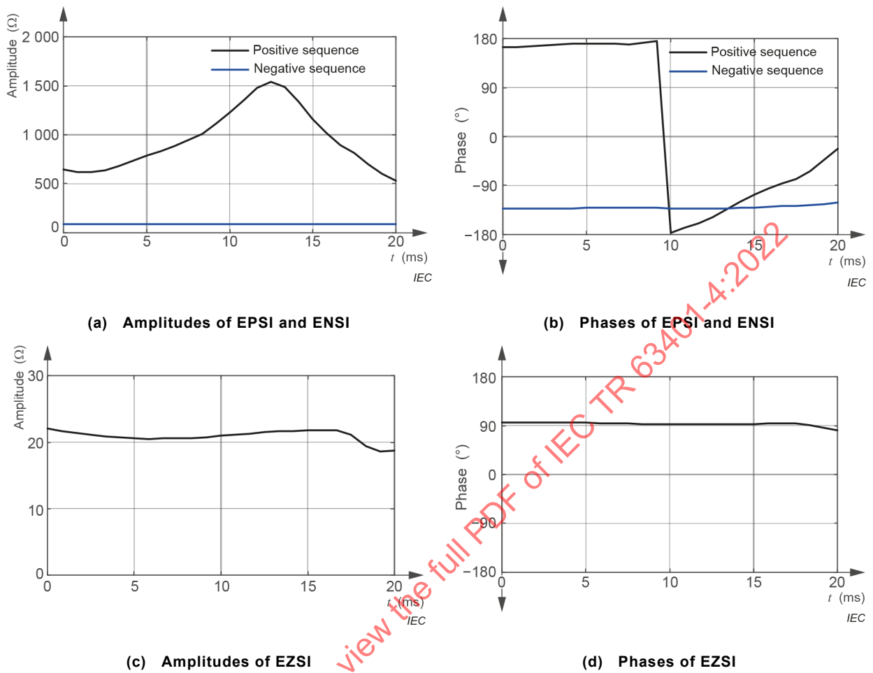
Figure 25 – The EPSI, ENSI, EZSI of wind farm including only DFIG based WTs
