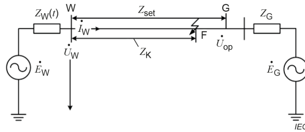
(a) Full fault network
