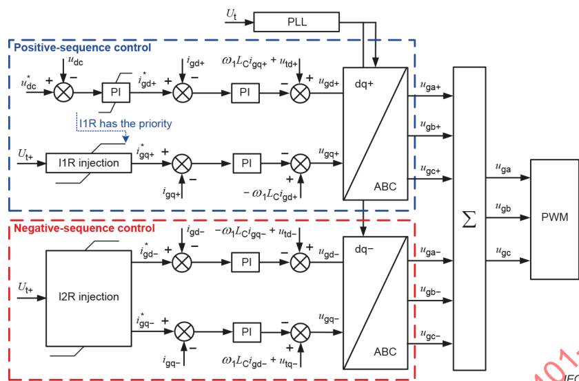
Figure 14 – Diagram of positive- and negative-sequence AC current control strategy of GSC for complying I1R and I2R injection requirements
