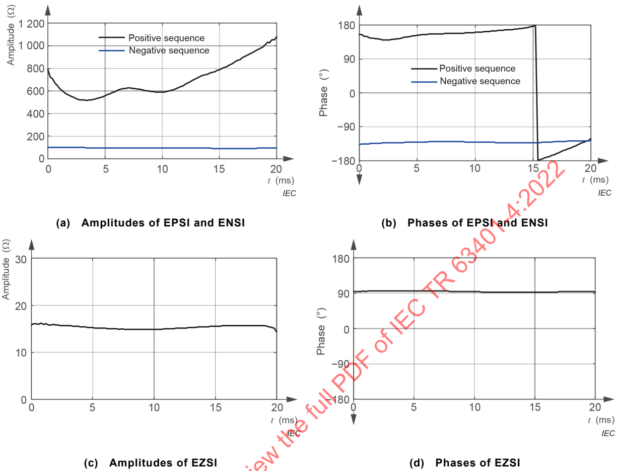
Figure 24 – The EPSI, ENSI, EZSI of wind farm including both DFIG and PMSG based WT's
