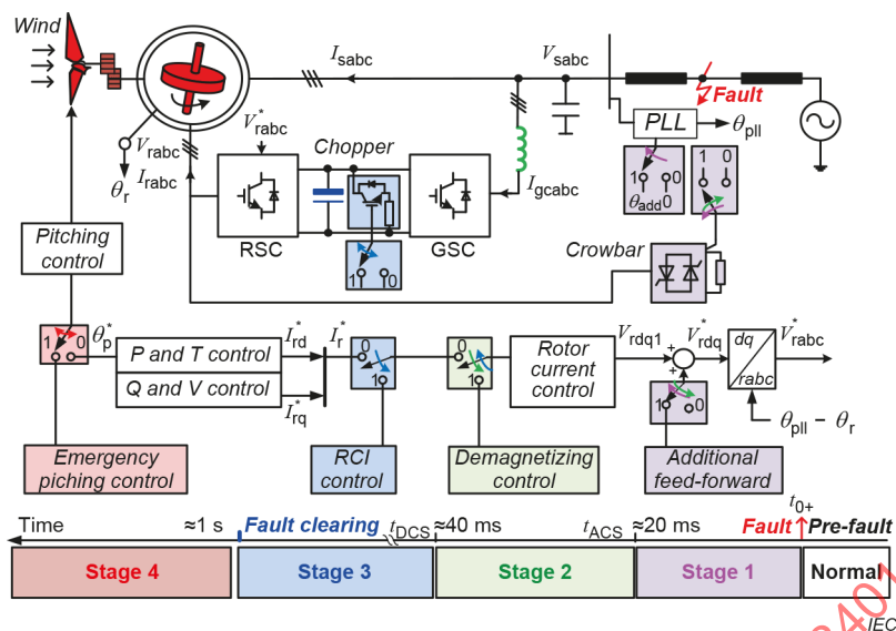
Figure 18 – FRT solutions of a DFIG-based WT during grid fault
