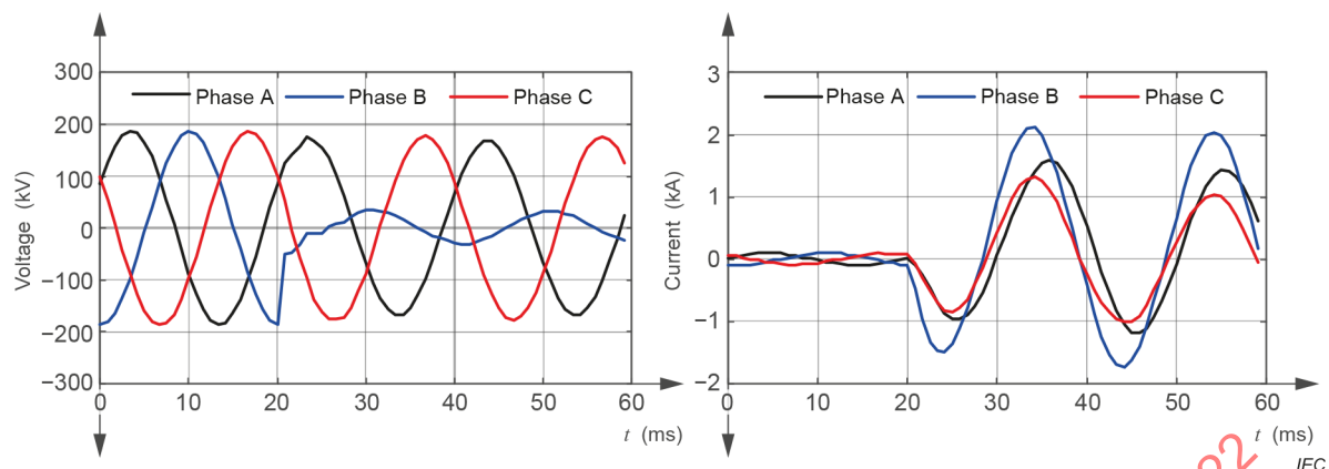
Figure 23 – The u_D and i_D recorded when BG fault occurs at point F1
