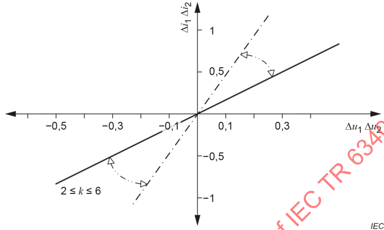
Figure 9 – Requirements of the reactive current according to VDE-AR-N 4120
