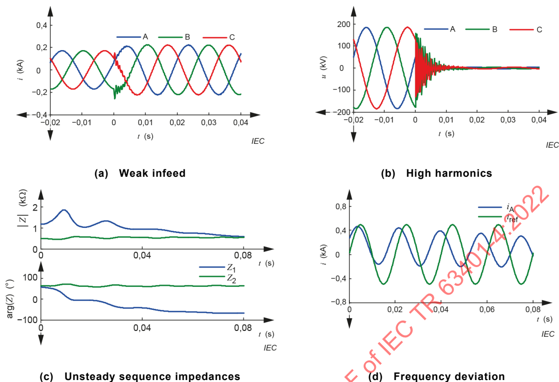
Figure 27 – General fault characteristics of wind power system
