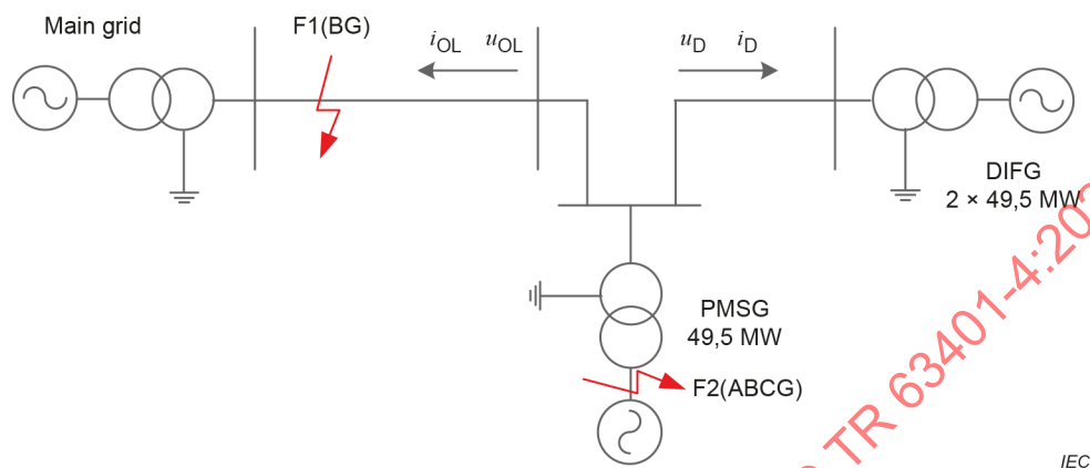
Figure 21 – The topology of wind farm integrated to power grid in Shanxi Province
