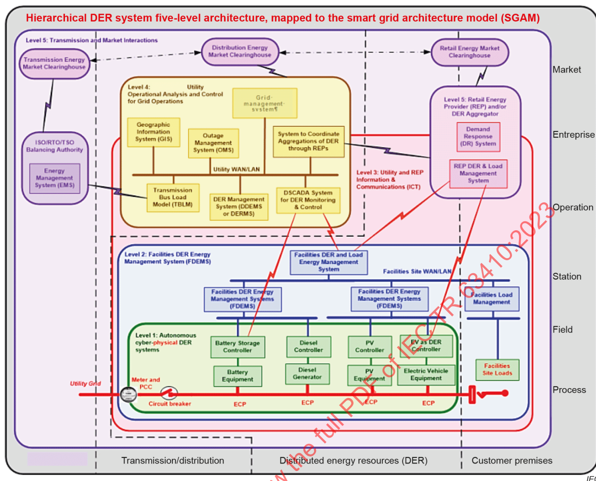
Figure 10 – Example of a hierarchical DER system five-level architecture in SGAM format
