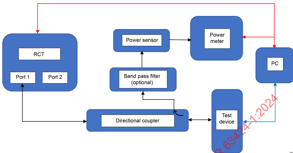
Figure B.1 – Typical single RAT power measurement configuration with optional band pass filter for directional coupler cross-coupling isolation
