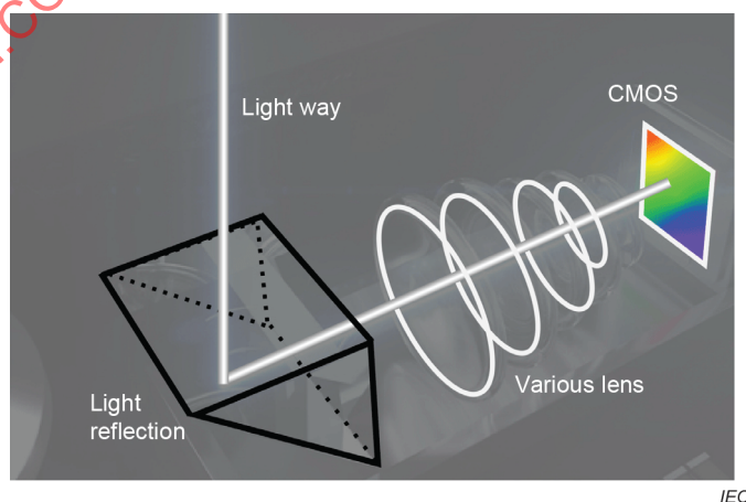
Figure 4 – Example of camera lens structure to reduce the prominent shape
