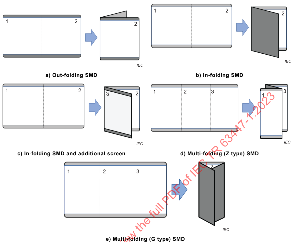
Figure 10 – Various SMD folding types
