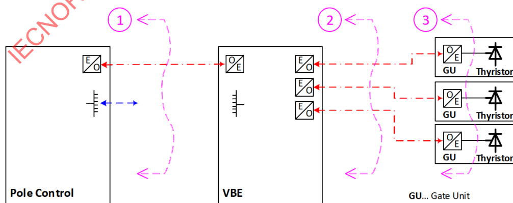
Figure 4 – Interfaces between HVDC C&P, VBE and thyristor valves
