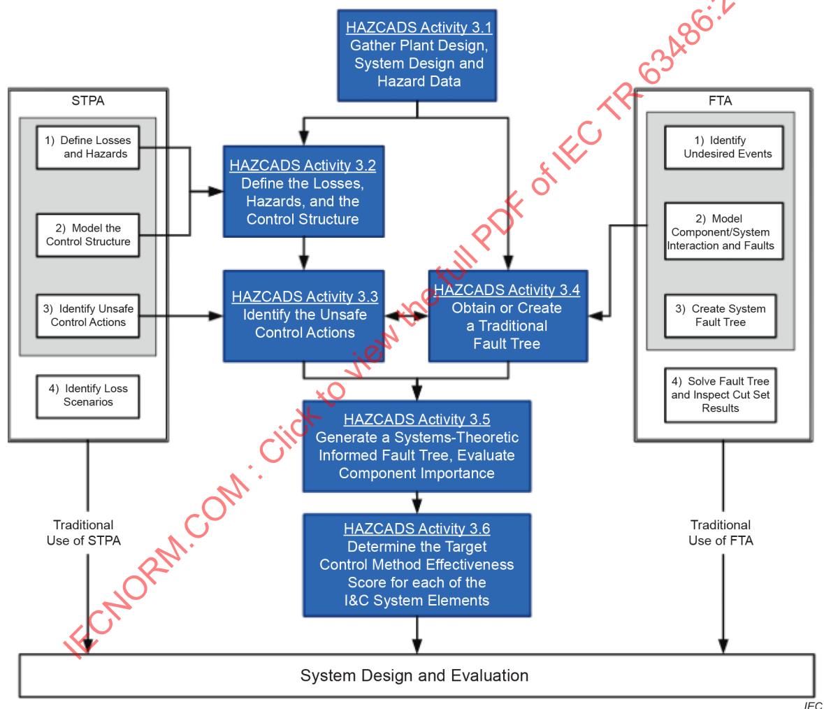
Figure F.1 – Overview of HAZCADS method (See Reference documents, EPRI 2018)
