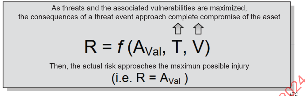
Figure E.1 – HTRA risk formula (Figure B-4 of [8])
