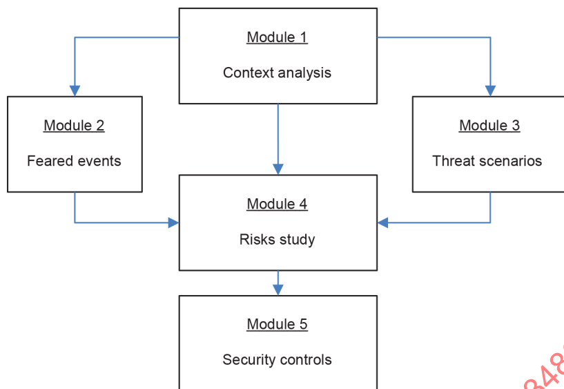
Figure C.1 – EBIOS 2010 process overview
