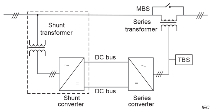
Figure 4 – Energizing test of the shunt converter
