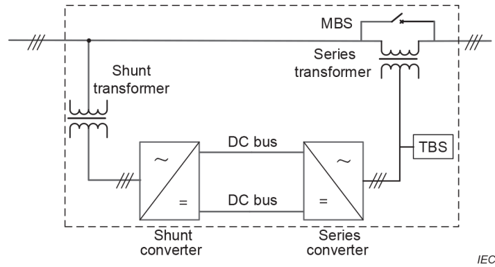
Figure 8 – System function and performance tests of UPFC
