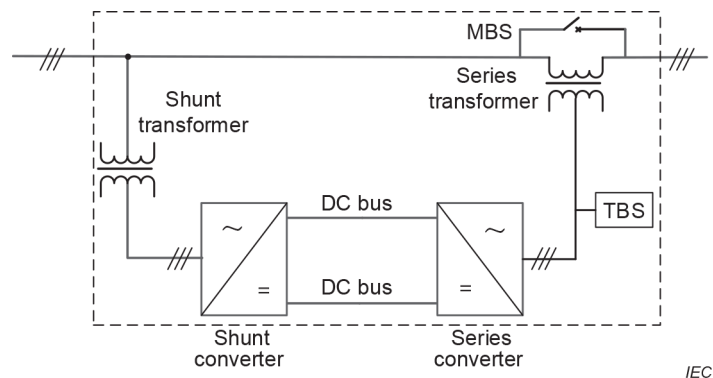
Figure 11 – Trial operation
