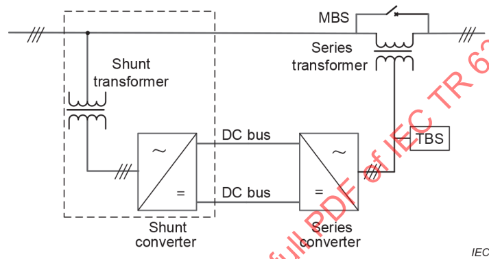
Figure 9 – Other operation mode tests – STATCOM mode
