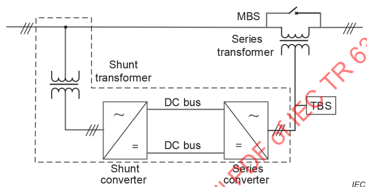
Figure 5 – Energizing test of the series converter
