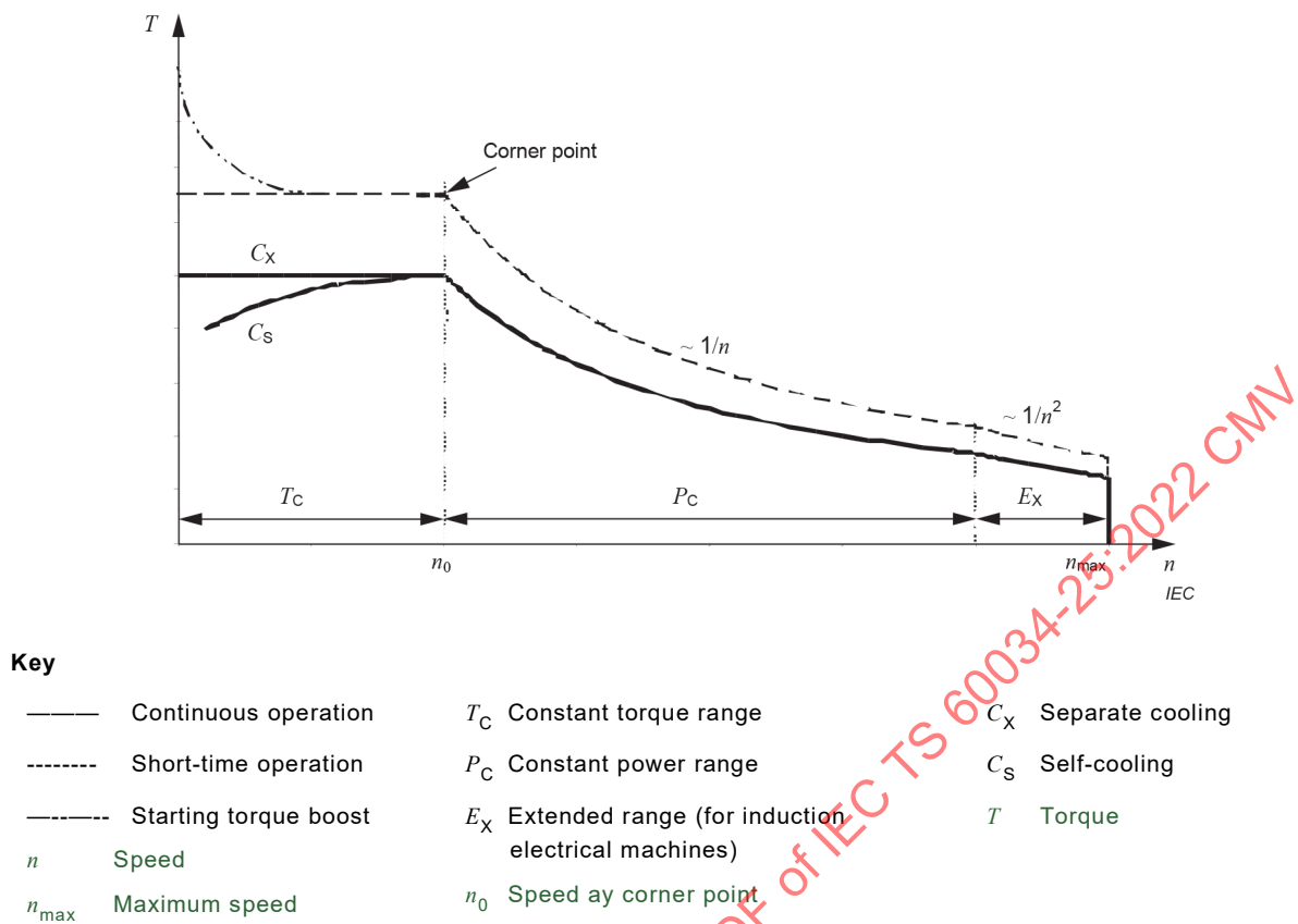
Figure 1 – Torque/speed capability
