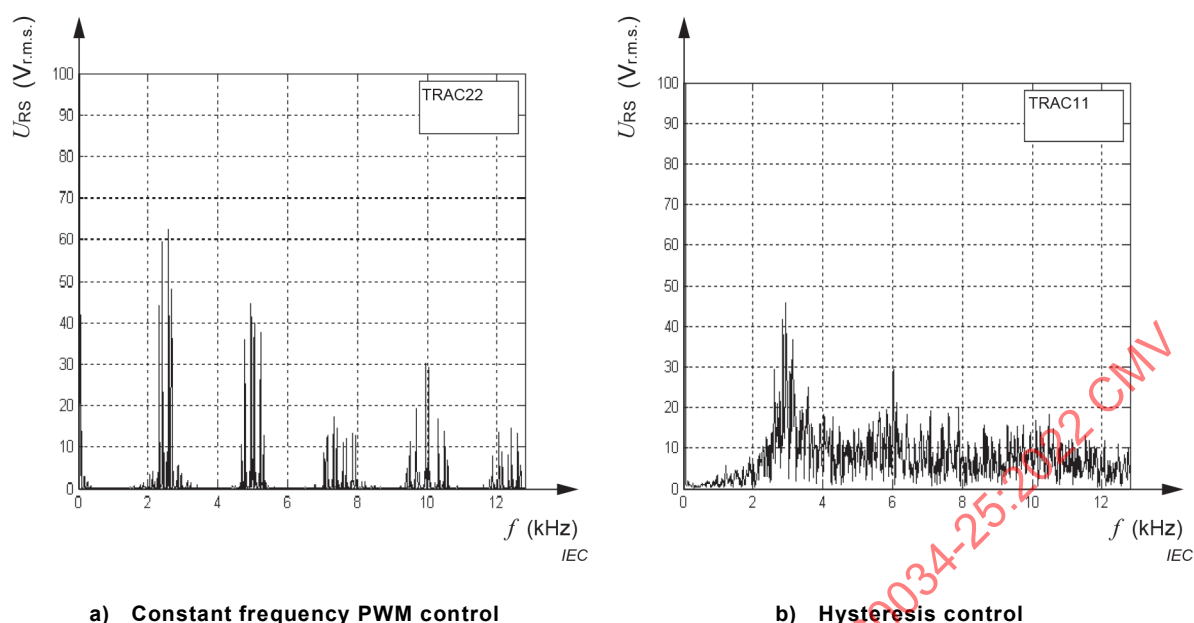
Figure B.2 – Typical output voltage frequency spectra of converter output voltage for a constant frequency PWM control versus hysteresis control
