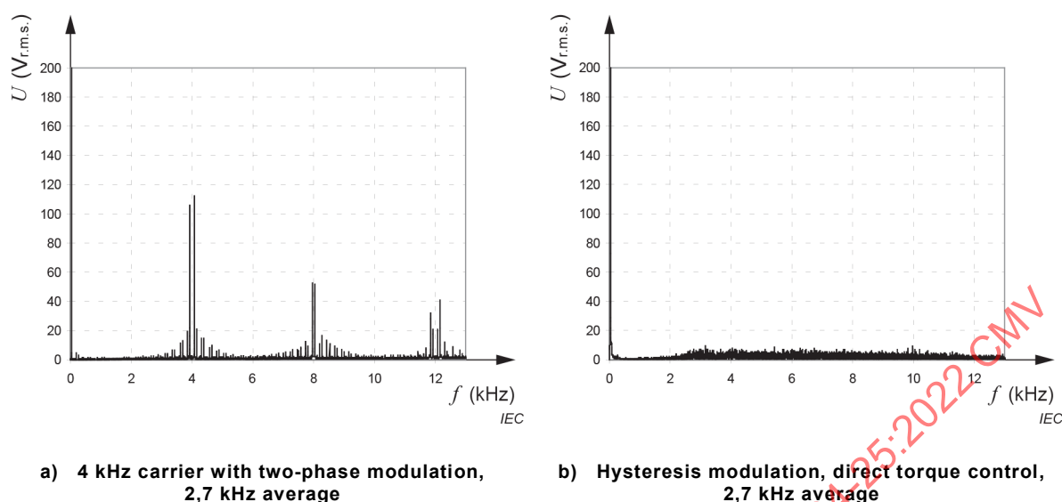
Figure B.4 – Typical spectra of converter output voltage frequency spectra for a two-phase modulated control versus hysteresis modulation
