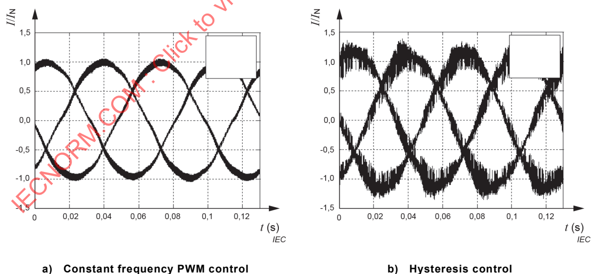
Figure B.5 – Typical time characteristics of electrical machine current for a Constant frequency PWM control versus hysteresis control
