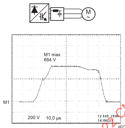
Figure 30b – Output d/dt filter
