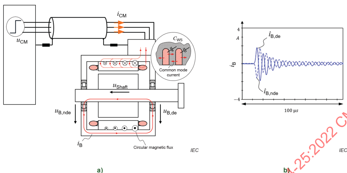
Figure 20 – Principle of circulating currents formation
