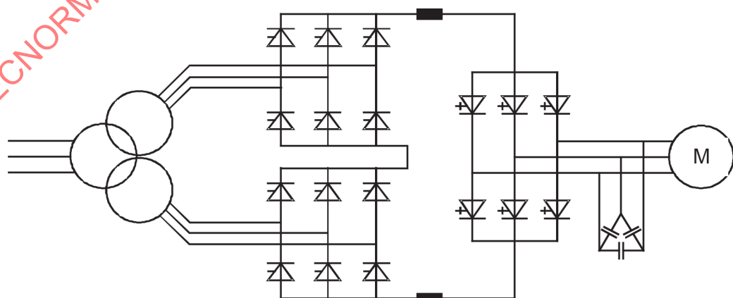
Figure 39 – Schematic of pulsed current source converter
