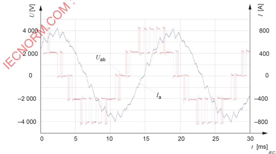
Figure 32 – Output voltage and current from typical three-level converter
