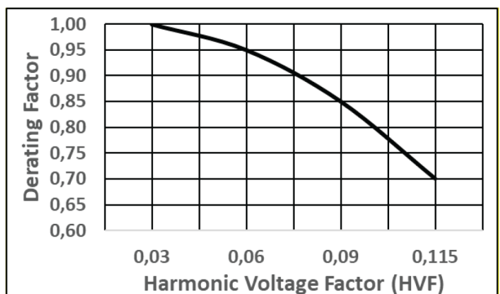
Figure D.1 – Derating curve for harmonic voltages
