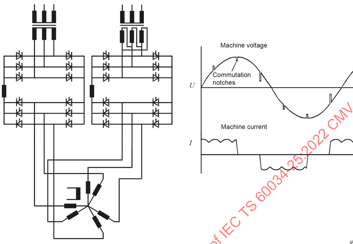
Figure 38 – Schematic and voltage and current waveforms for a synchronous electrical machine supplied from a current source converter
