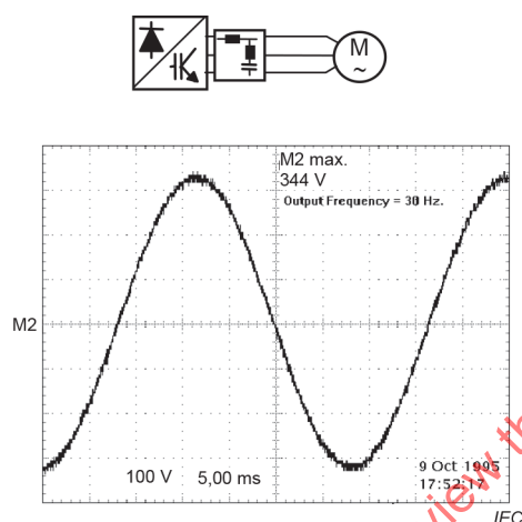
Figure 30c – Sinusoidal filter
