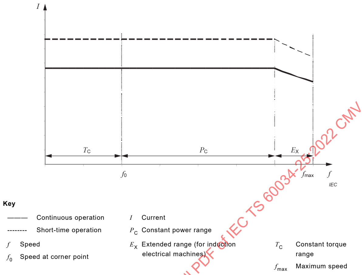
Figure 2 – Current required by motor
