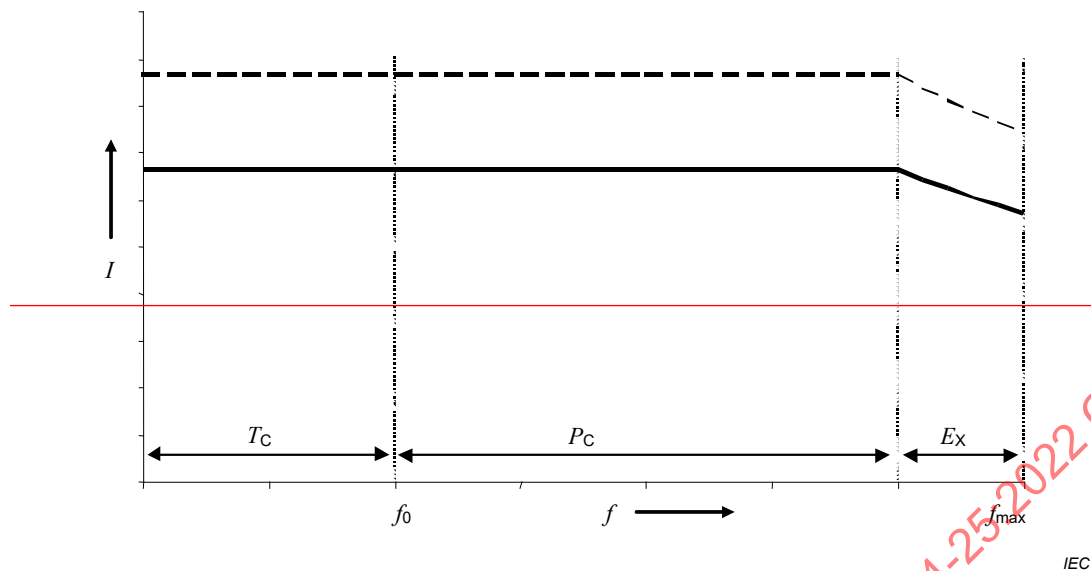
Figure 2 – Converter output current
