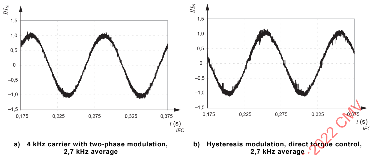
Figure B.6 – Typical time characteristics of electrical machine current for a two-phase modulated control versus hysteresis modulation
