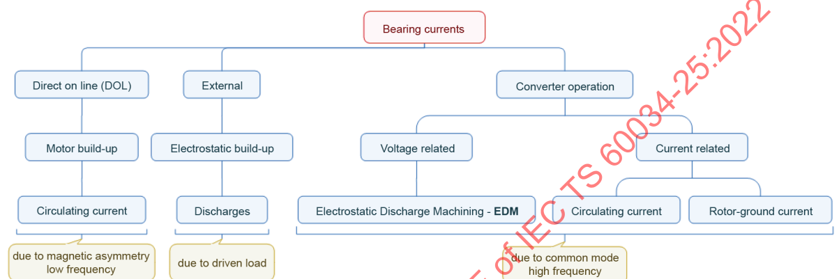
Figure 15 – Classification of bearing currents
