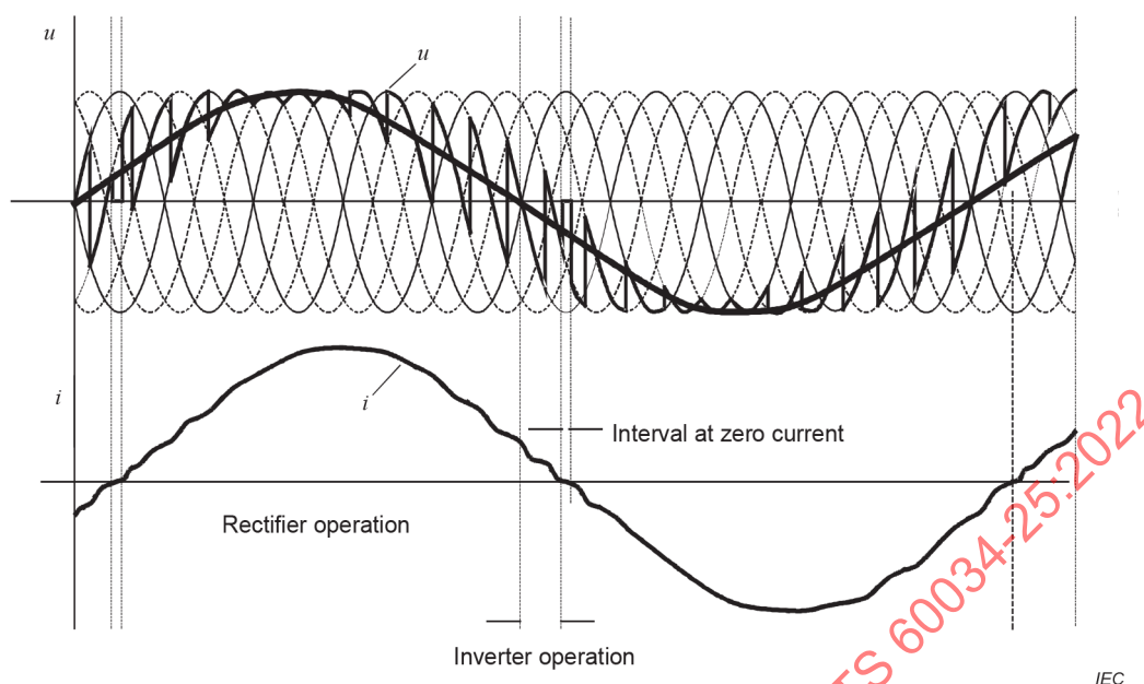
Figure 42 – Voltage and current waveforms of a cyclo-converter
