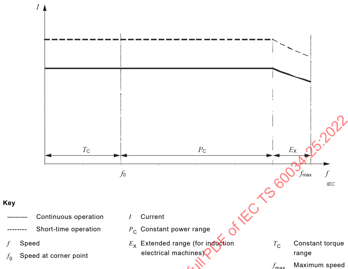
Figure 2 – Current required by motor
