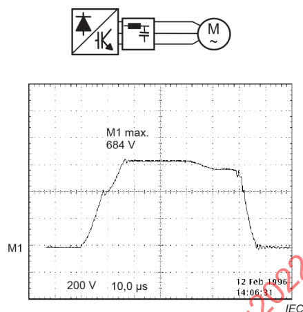
Figure 30b – Output dU/dt filter
