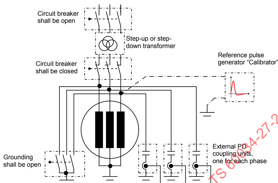
Figure 4 – Measuring object, during normalization
