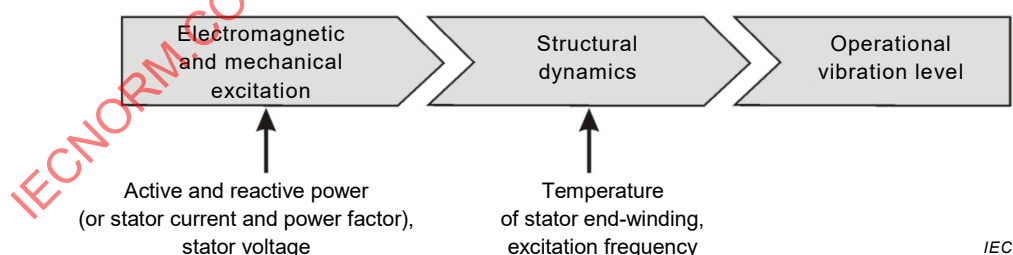
Figure 4 – Simplified cause effect chain of stator end-winding vibration and influencing operational parameters
