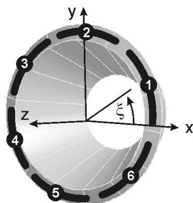
Figure A.7 – Sensors for the measurement of global vibration level centred in the winding zones
