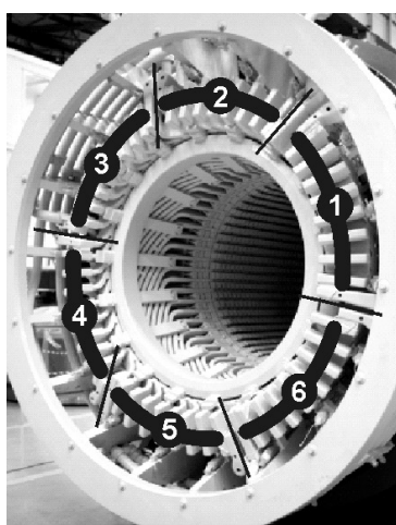
Figure A.7 – Sensors for the measurement of global vibration level centred in the winding zones
