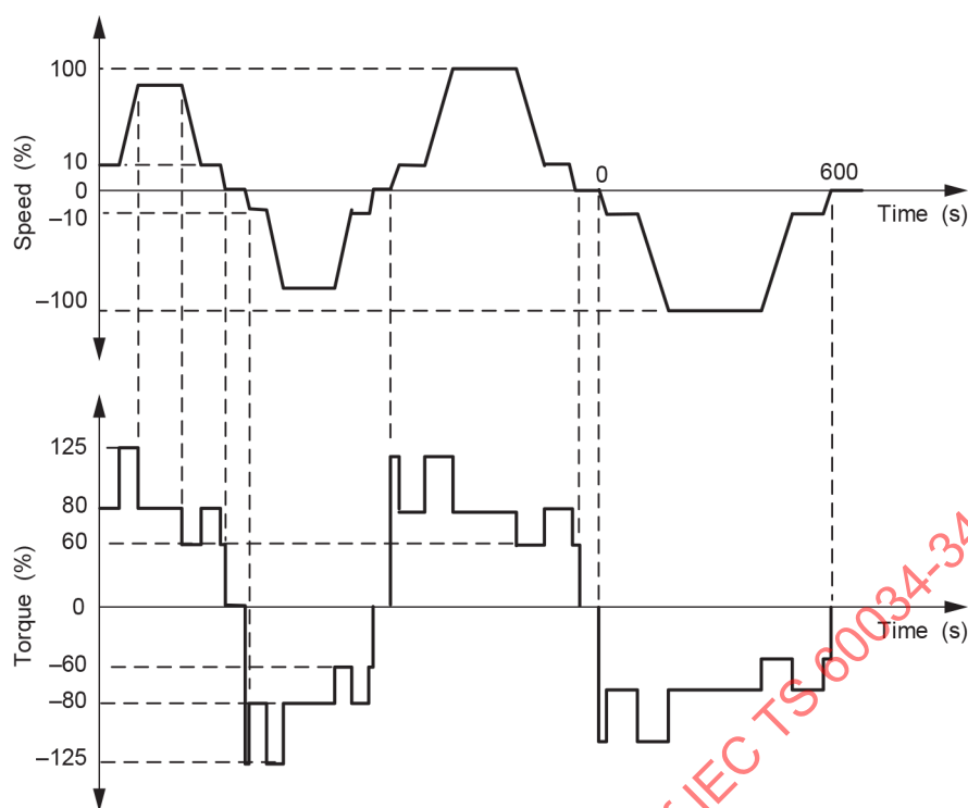
Figure B.5 – Typical rolling operation pattern for cold reversing rolling mills
