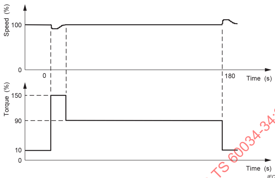
Figure B.4 – Typical rolling operation pattern for hot continuous rolling for wire and rod mills
