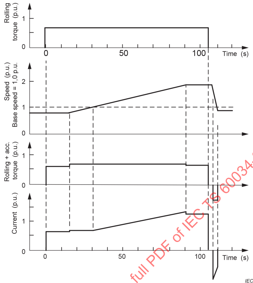
Figure C.4 – Torque, speed and current deviation in one rolling cycle for hot strip mill finishing motor
