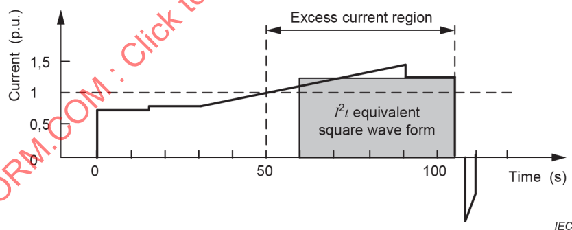
Figure C.3 – Equivalent rectangular current waveform introduction
