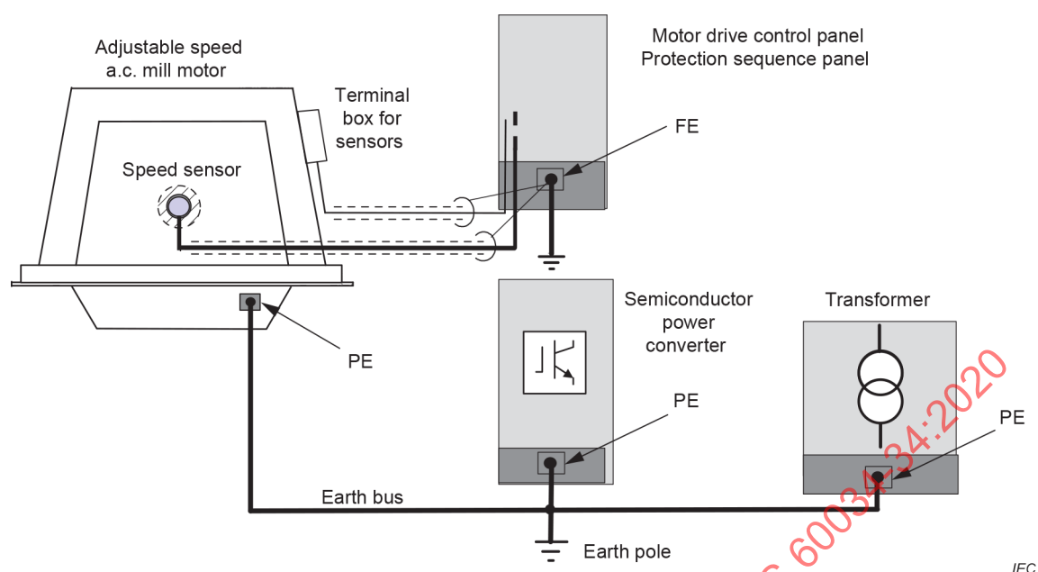
Figure 8 – Example of protective earthing and functional earthing
