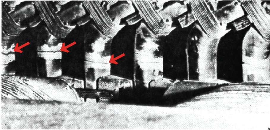
Figure D.1 – Example of stator coil insulation surface crack caused by repetitive mechanical stress
