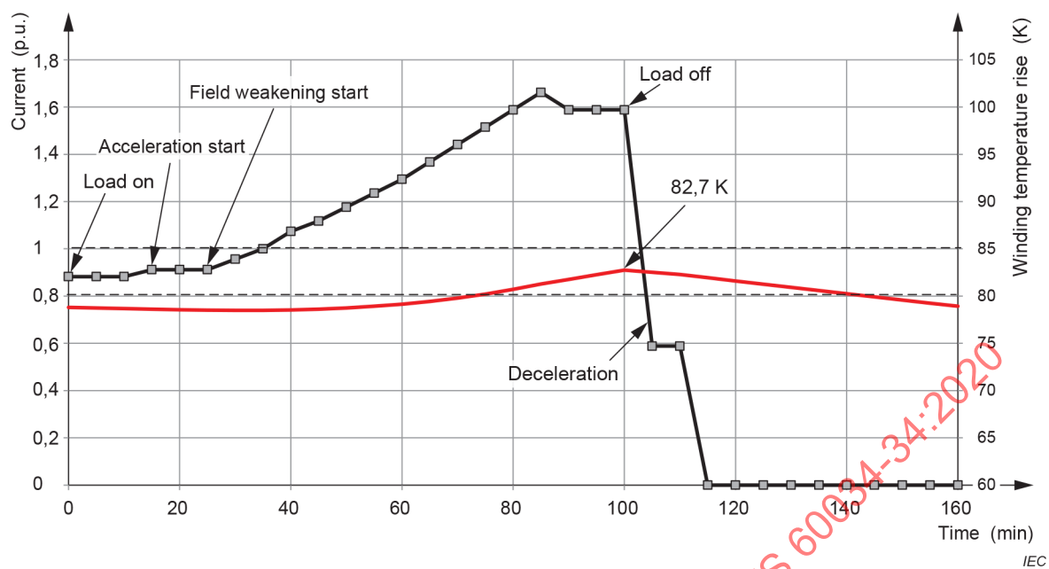
Figure C.5 – An example of winding temperature deviation estimation in one rolling cycle by the precise method
