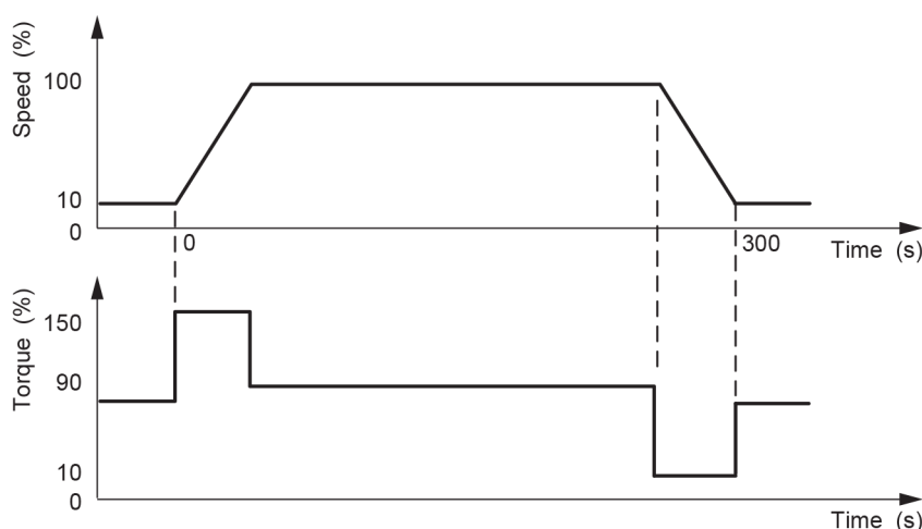
Figure B.6 – Typical rolling operation pattern for cold continuous rolling
