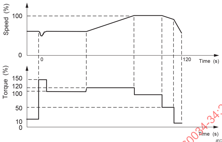
Figure B.2 – Typical rolling operation for hot continuous rolling of sheet strip
