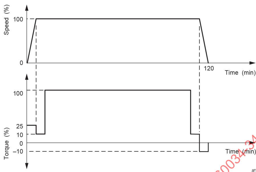
Figure B.3 – Typical rolling operation pattern for continuous caster connected hot continuous rolling for sheet strip
