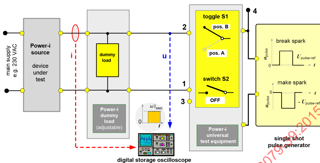
Figure A.4 – Basic principle of the equipment for the determination of the response time t_{\text{resp-source}}
