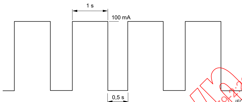
Figure 16 – Series of four rectangular pulses of unidirectional current
