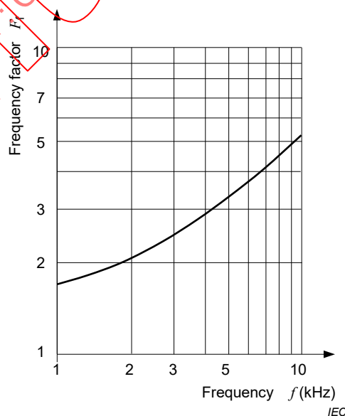
Figure 5 – Variation of the threshold of let-go within the frequency range 1 000 Hz to 10 000 Hz
