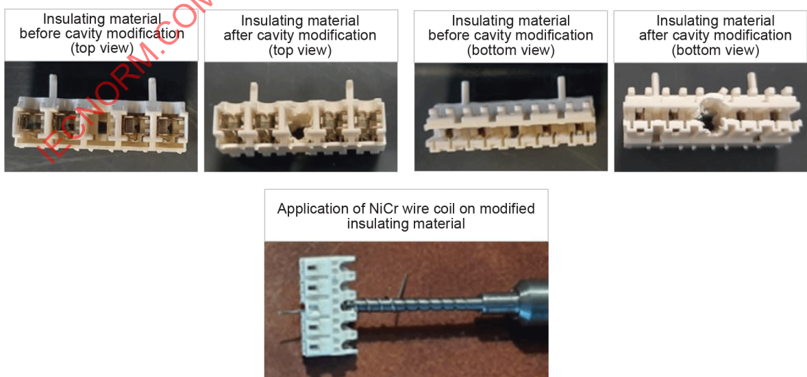
Figure B.4 – Example 3 of NiCr wire coil application
