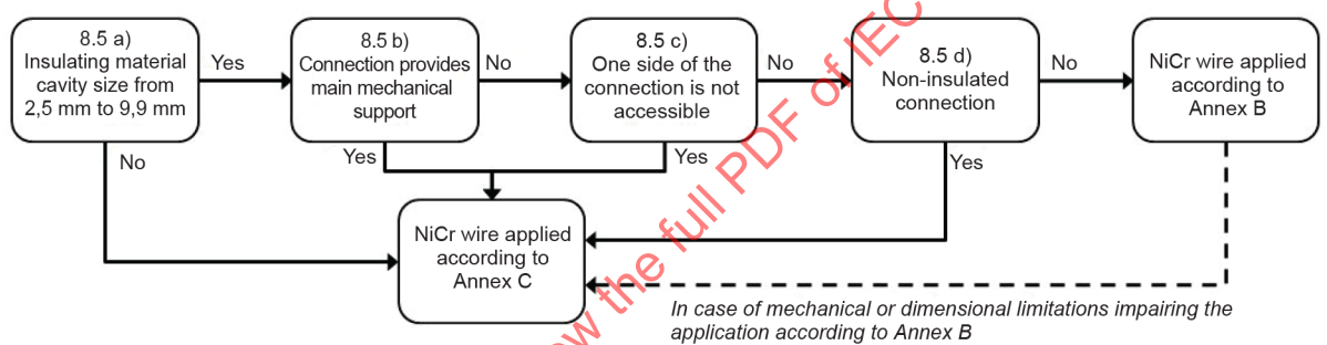
Figure 3 – NiCr wire application methodology selection flow-chart
