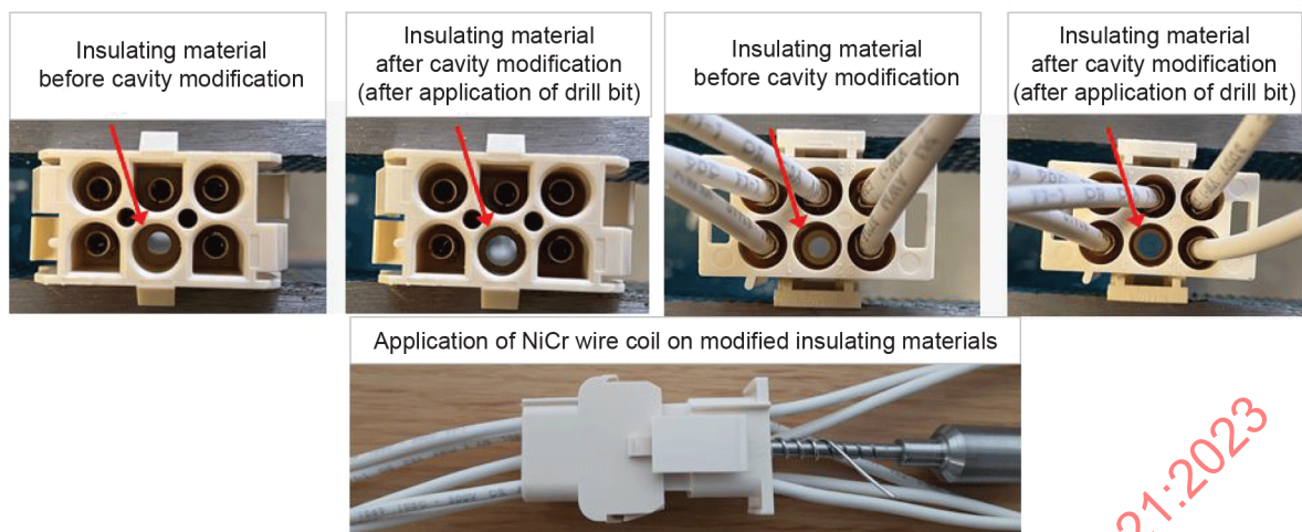
Figure B.2 – Example 1 of NiCr wire coil application
