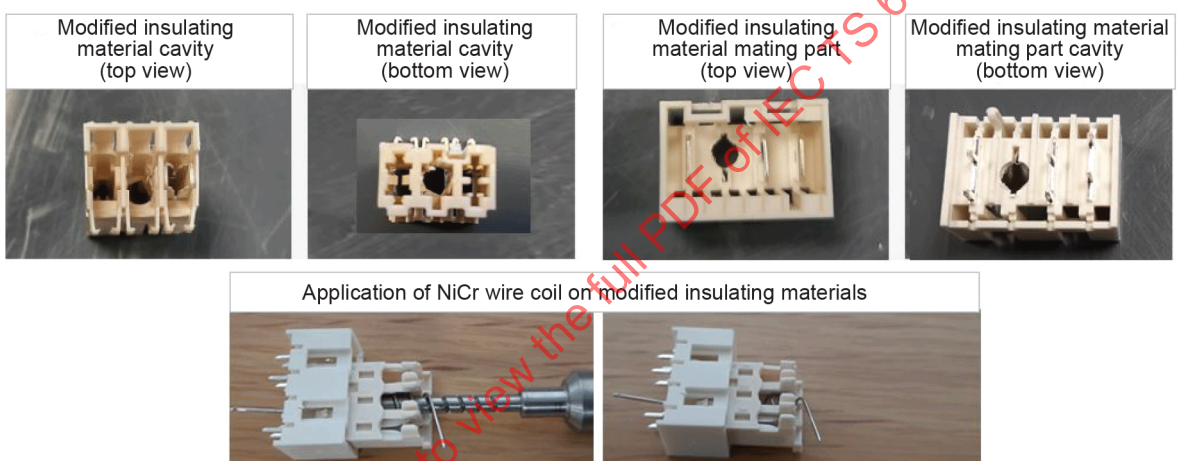
Figure B.3 – Example 2 of NiCr wire coil application
