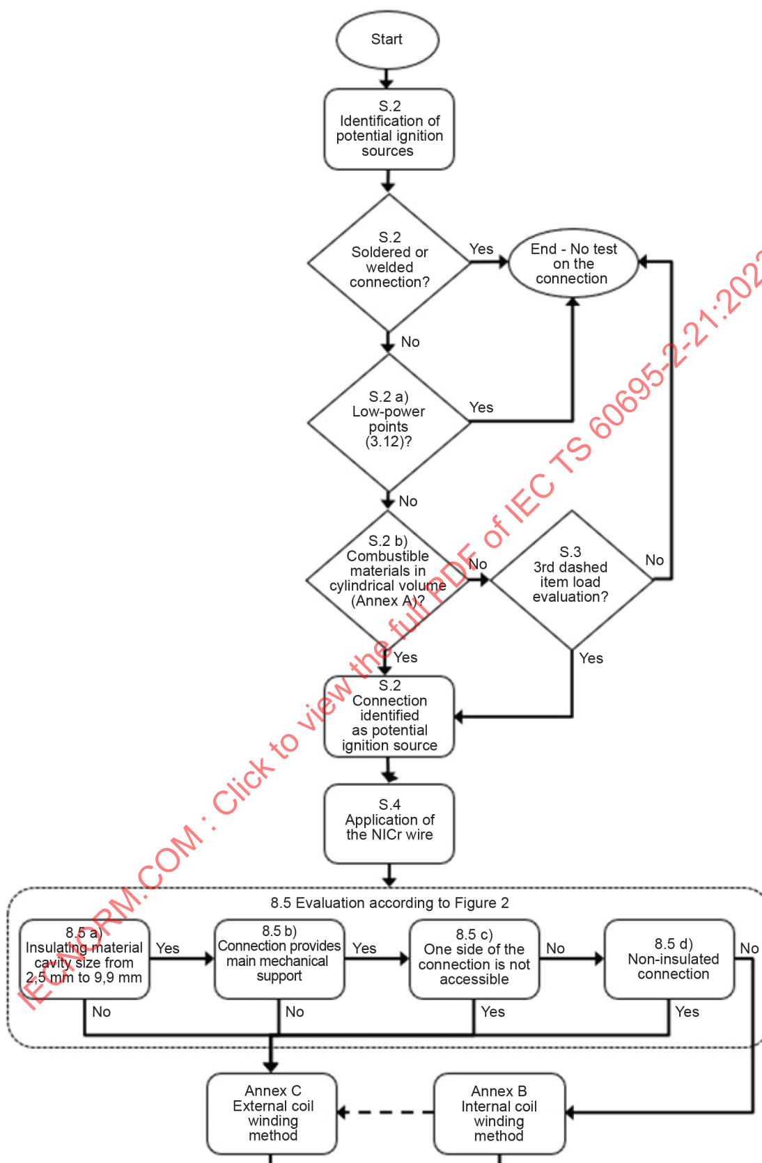
Figure 1 – Test procedure flow-chart (1 of 2)
