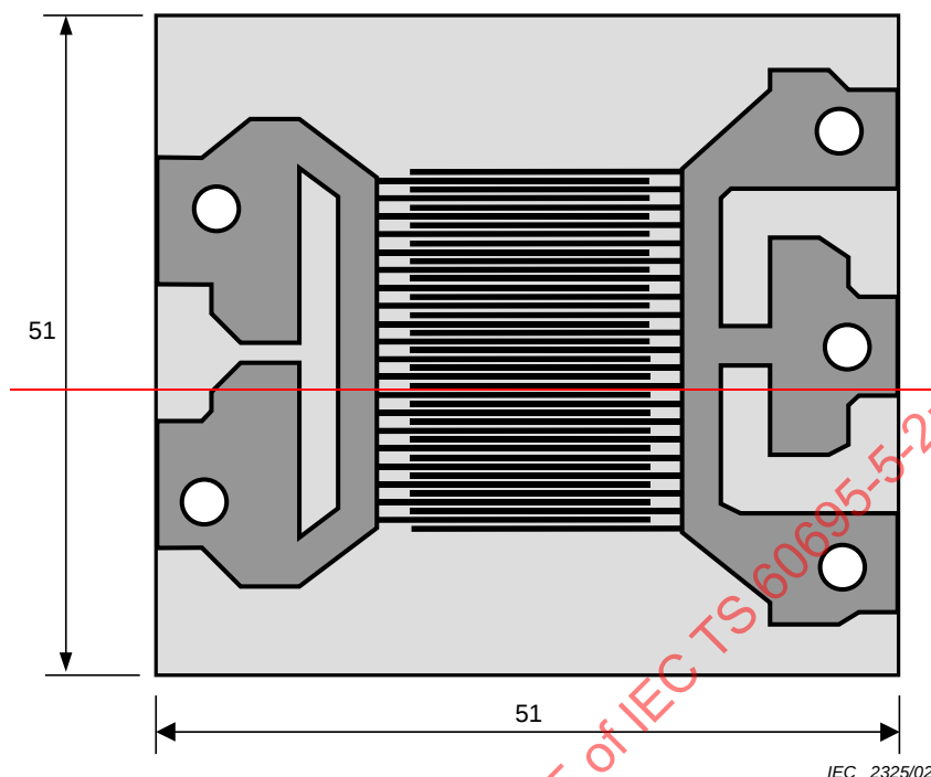
Figure 3 — Interdigitated leakage current target
