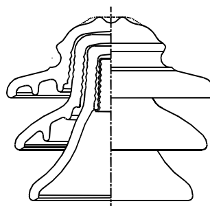
Figure 6b – Multi-element pin insulator
