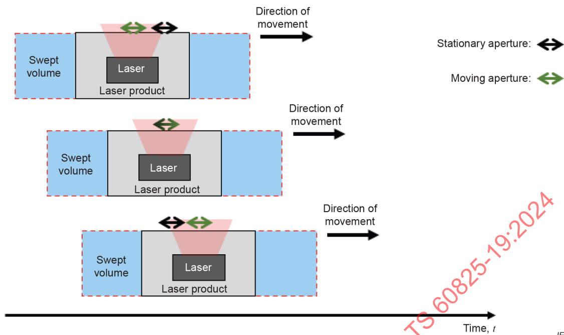
Figure A.5 – Position of the stationary and the moving aperture over time when evaluating neighbouring platforms
