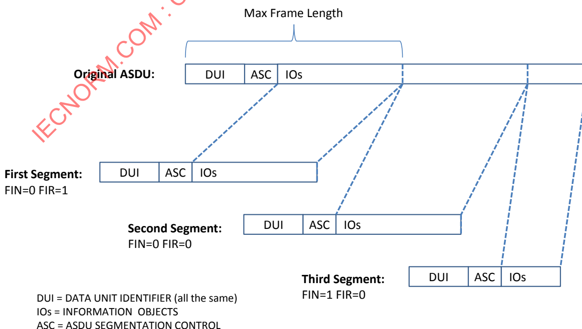
Figure 2 – Segmenting extended ASDUs
