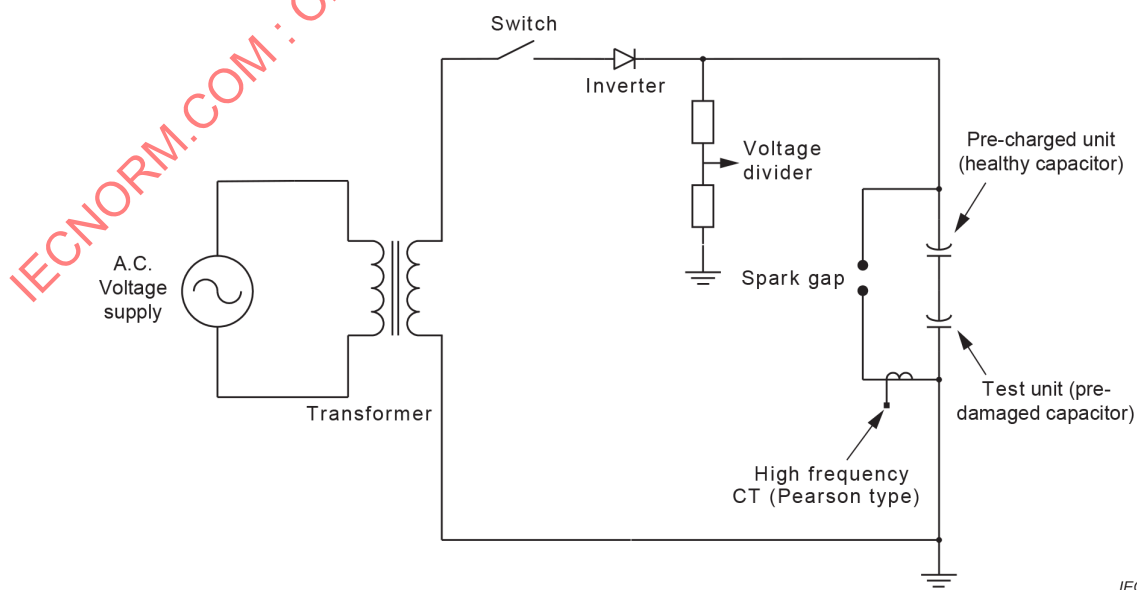
Figure 3 – Electric circuit for the discharge test
