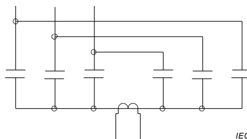
Figure 6 – Double-star connection with ungrounded neutral
