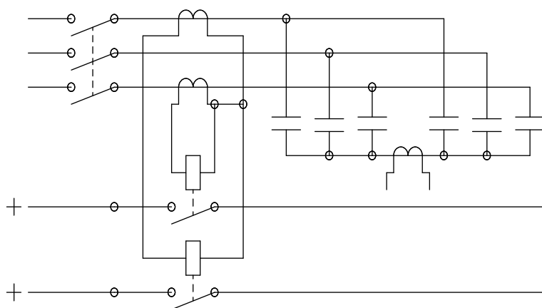
Figure 10 – Line overcurrent relays for capacitor bank, ungrounded
