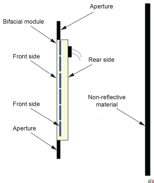
Figure 2 – Scheme of a bifacial PV module and the required non-irradiated background and aperture
