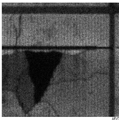
Figure 7 – Images of regions of multicrystalline silicon solar cells with three SNR_{50} values as labeled
