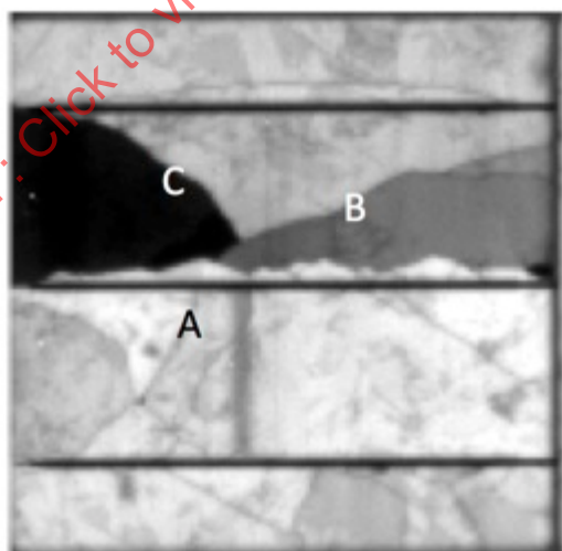
Figure C.1 – Single cell region of a module with 0,1 \times I_{sc} applied showing crack types, as labeled
