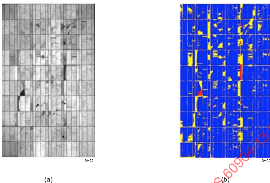
Figure C.3 – Example of quantifying solar cell cracks in photovoltaic modules: (a) EL image produced with 0,1 \cdot I_{sc} forward bias current, and (b) image of regions considered damaged
