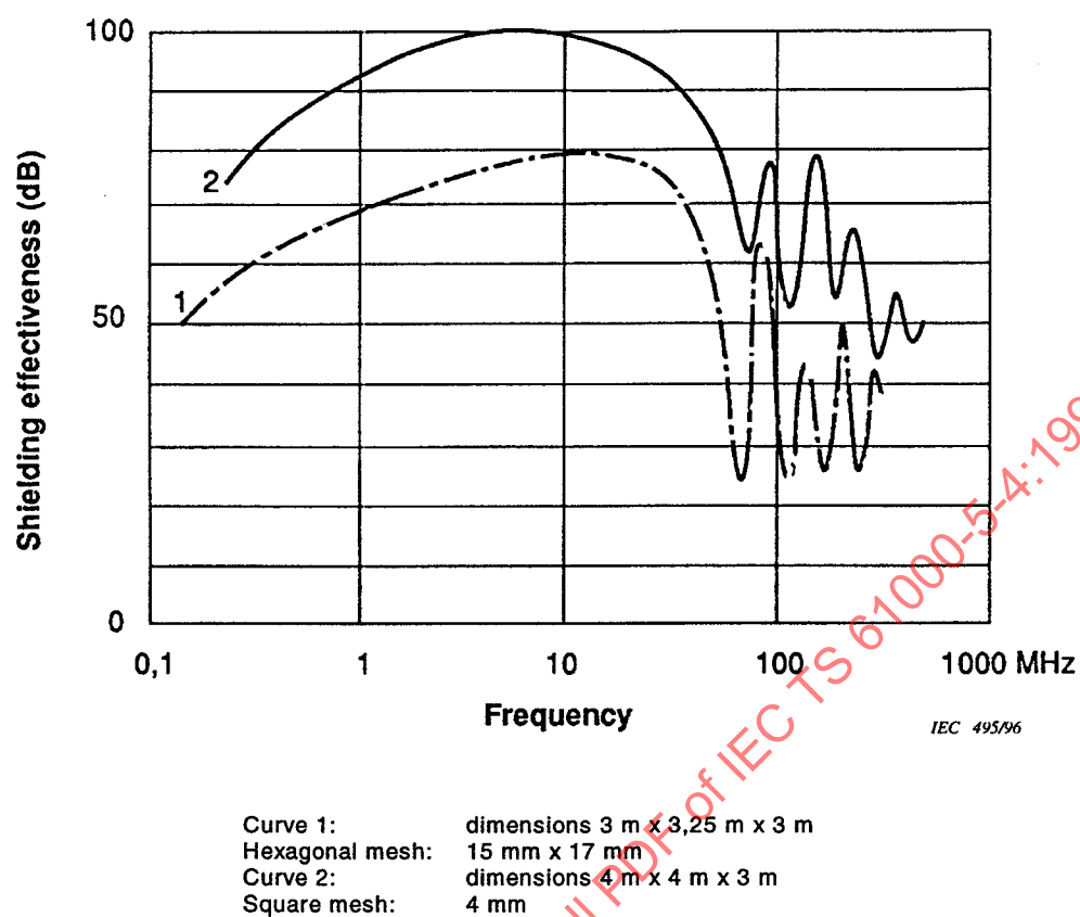
Figure 1 – Typical plane wave attenuation for double-wall cages
