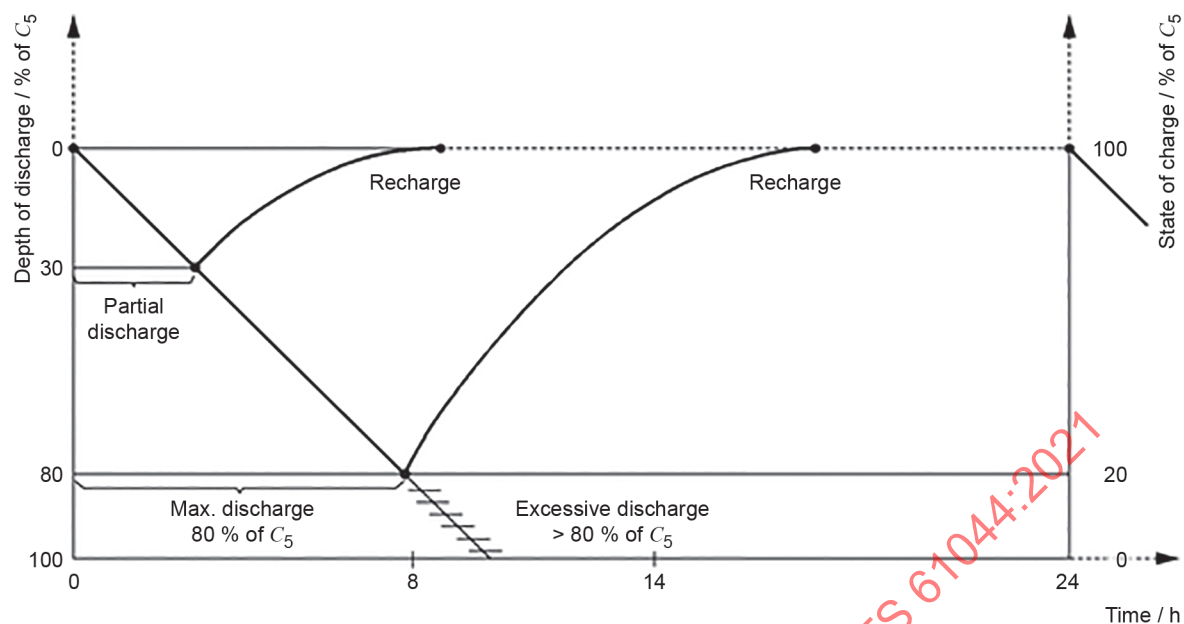
a) Schematic pattern of a 24 h (daily) normal discharge and charge duty of a vented lead-acid battery
