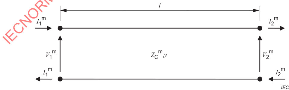
Figure 8 – Transmission line system
