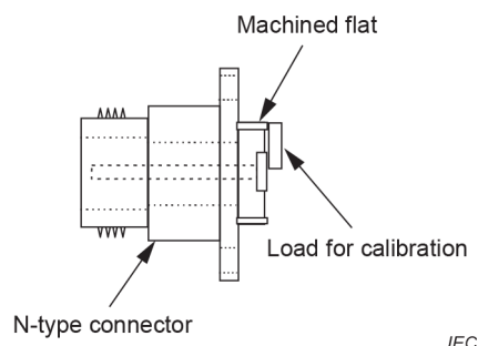
Figure 16 – Solution for calibration of reference loads
