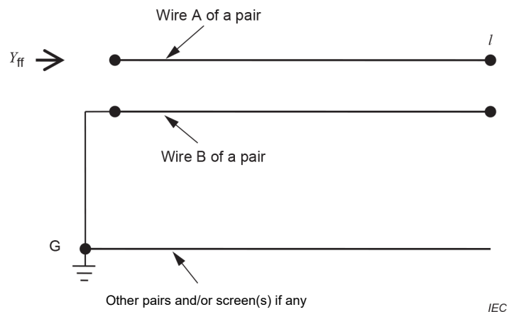
a) Measurement mode a: Y_{ff}
