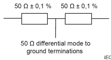
Figure 17 – Resistor termination networks
