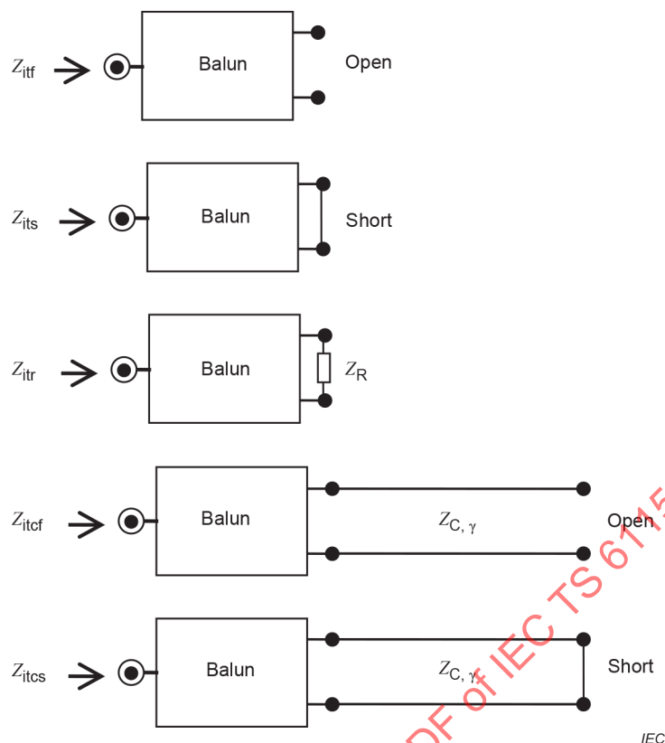
Figure 4 – Measurement configurations
