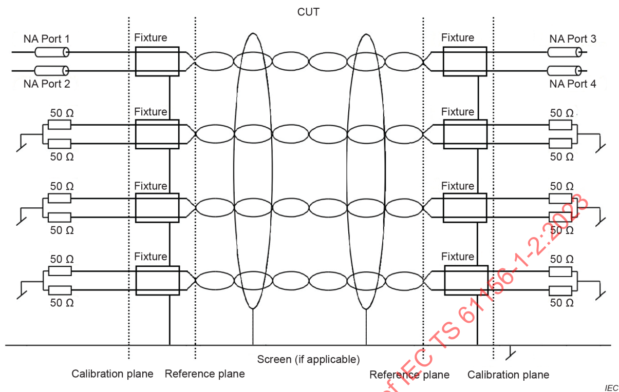
Figure 18 – Insertion loss and EL TCTL
