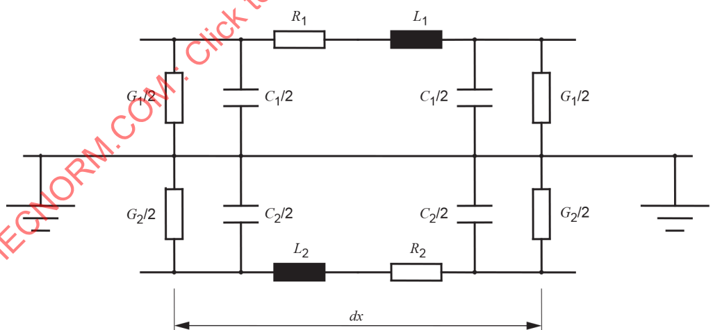
Figure 11 – Circuit of an infinitesimal element of a symmetric pair
