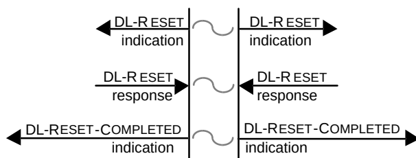
Figure 56 — Sequence of primitives in a Peer DLS-provider initiated Reset
