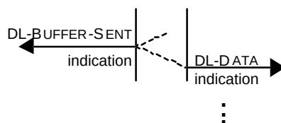
Figure 50 — Sequence of primitives for a Publisher to Subscribers buffer to queue data transfer
