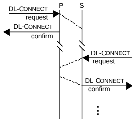
Figure 20 — Multi-peer DLC/DLCEP establishment using known DLCEP addresses initiated first by the Publishing DLS-user
