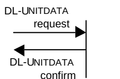
Figure 68 — Sequence of primitives for an unsuccessful connectionless-mode unitdata transfer
