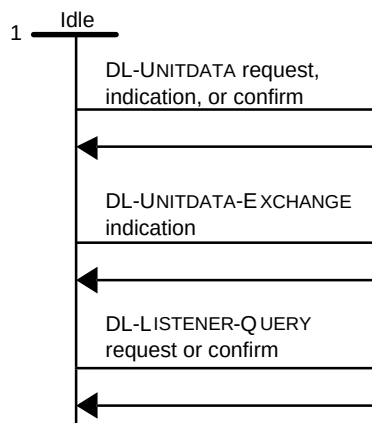
Figure 65 — State transition diagram for sequences of connectionless-mode primitives at one DLSAP
