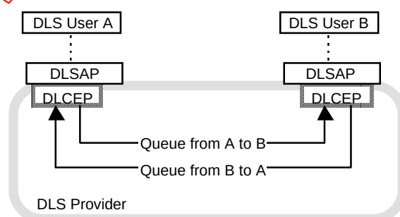
Figure 8 — OSI abstract queue model of a peer DLC between a pair of DLS-users
