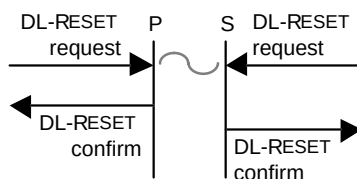
Figure 55 — Sequence of primitives in a simultaneous Multi-peer DLS-users initiated Reset
