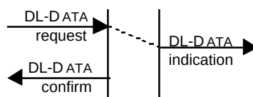
Figure 44 — Sequence of primitives for an Ordered or Unordered peer-to-peer, or an Unordered subscriber-to-publisher queue-to-queue data transfer
