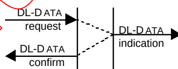
Figure 43 — Sequence of primitives for a Classical or Disordered peer-to-peer queue to queue data transfer
