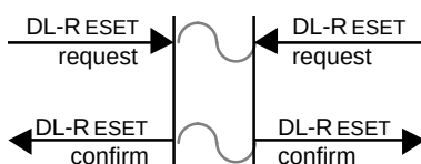
Figure 54 — Sequence of primitives in a simultaneous Peer DLS-users initiated Reset
