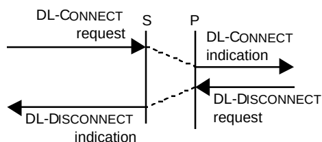
Figure 35 — Sequence of primitives in a Publishing DLS-user rejection of a DLC/DLCEP establishment attempt
