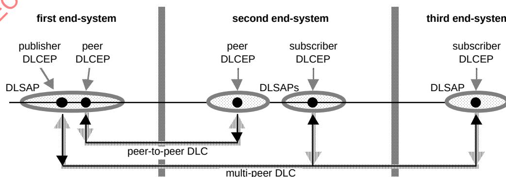
Figure 7 — Peer-to-peer and multi-peer DLCs and their DLCEPs
