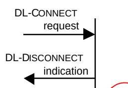
Figure 37 — Sequence of primitives in a DLS-provider rejection of a DLC/DLCEP establishment attempt
