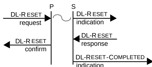
Figure 60 — Sequence of primitives in a simultaneous Publishing DLS-user and DLS-provider initiated Reset
