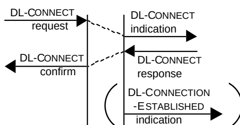
Figure 19 — Multi-peer DLC/DLCEP establishment initiated by a Subscribing DLS-user
