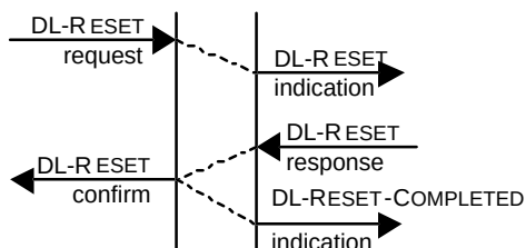
Figure 51 — Sequence of primitives in a Peer DLS-user initiated Reset
