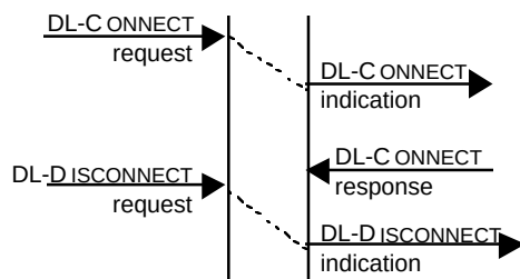
Figure 40 — Sequence of primitives in a DLS-user cancellation of a DLC/DLCEP establishment attempt: Peer DL-DISCONNECT indication arrives after DL-C ONNECT response is sent
