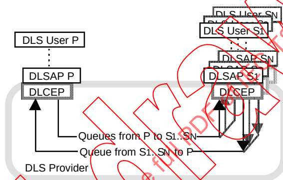
Figure 9 — OSI abstract queue model of a multi-peer DLC between a publishing DLS-user and a set of subscribing DLS-users
