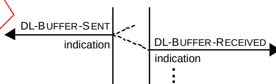
Figure 48 — Sequence of primitives for a Publisher to Subscribers buffer to buffer data transfer
