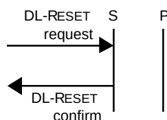
Figure 61 — Sequence of primitives in a simultaneous Subscribing DLS-user and DLS-provider initiated Reset
