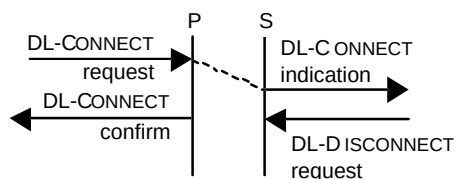
Figure 36 — Sequence of primitives in a Subscribing DLS-user rejection of a DLC/DLCEP establishment attempt
