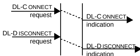
Figure 39 — Sequence of primitives in a DLS-user cancellation of a DLC/DLCEP establishment attempt: DL-DISCONNECT indication arrives before DL-CONNECT response is sent
