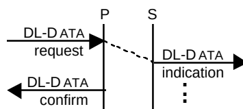
Figure 45 — Sequence of primitives for a publisher-to-subscribers queue to queue data transfer
