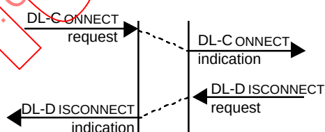
Figure 34 — Sequence of primitives in a Peer DLS-user rejection of a DLC/DLCEP establishment attempt
