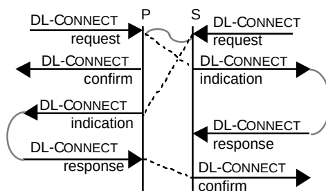
Figure 23 — Multi-peer DLC/DLCEP establishment initiated simultaneously by both Publishing and Subscribing DLS-users, resulting in a merged DLC
