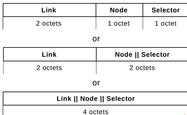
Figure A.3 — DL-address Alternative Structures
