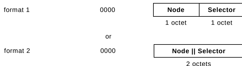
Figure 5 — SHORT DL-address field — alternative implicit structures
